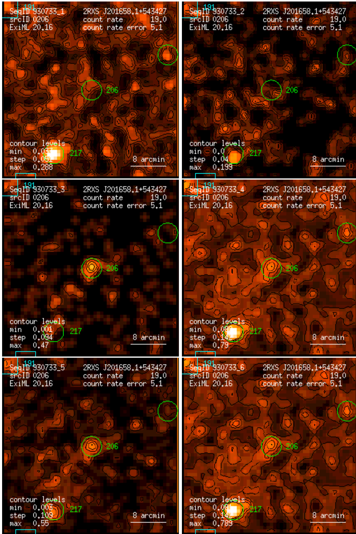
Figure 206: RASS 930733: detection 0206: band rate images, Gaussian filter: (1) PSPC channels 11 – 41, (2) 52 – 90, (3) 91 – 201, (4) 11 – 235, (5) 52 – 201, (6) 11 – 201. Broad band rates in counts/ks. Band rate contour levels in counts/ks/arcmin 2 .
