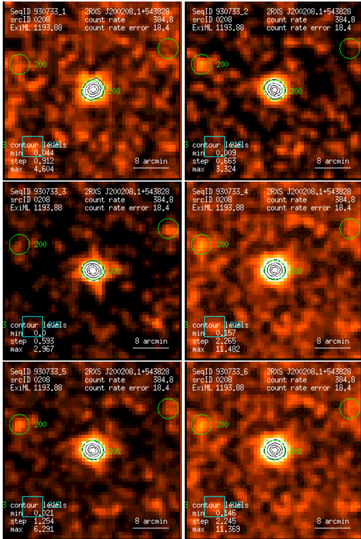
Figure 208: RASS 930733: detection 0208: band rate images, Gaussian filter: (1) PSPC channels 11 – 41, (2) 52 – 90, (3) 91 – 201, (4) 11 – 235, (5) 52 – 201, (6) 11 – 201. Broad band rates in counts/ks. Band rate contour levels in counts/ks/arcmin 2 .
