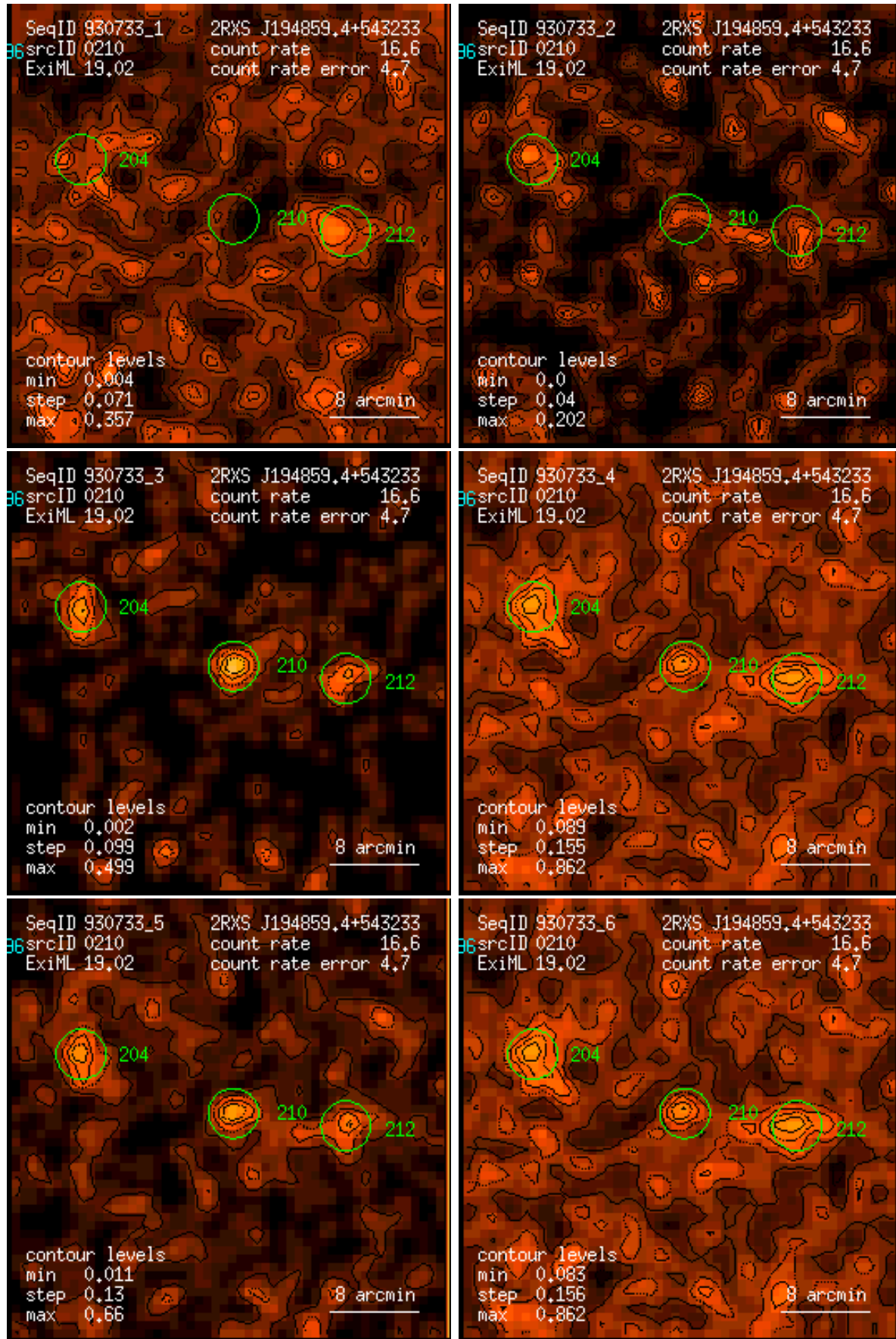
Figure 210: RASS 930733: detection 0210: band rate images, Gaussian filter: (1) PSPC channels 11 – 41, (2) 52 – 90, (3) 91 – 201, (4) 11 – 235, (5) 52 – 201, (6) 11 – 201. Broad band rates in counts/ks. Band rate contour levels in counts/ks/arcmin 2 .
