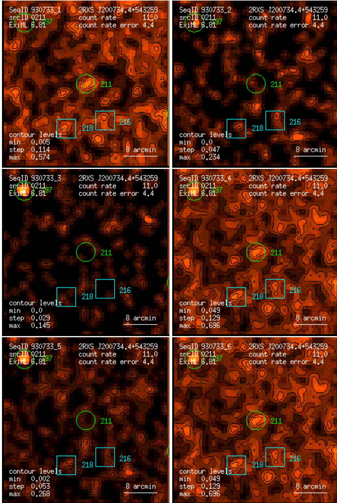
Figure 211: RASS 930733: detection 0211: band rate images, Gaussian filter: (1) PSPC channels 11 – 41, (2) 52 – 90, (3) 91 – 201, (4) 11 – 235, (5) 52 – 201, (6) 11 – 201. Broad band rates in counts/ks. Band rate contour levels in counts/ks/arcmin 2 .
