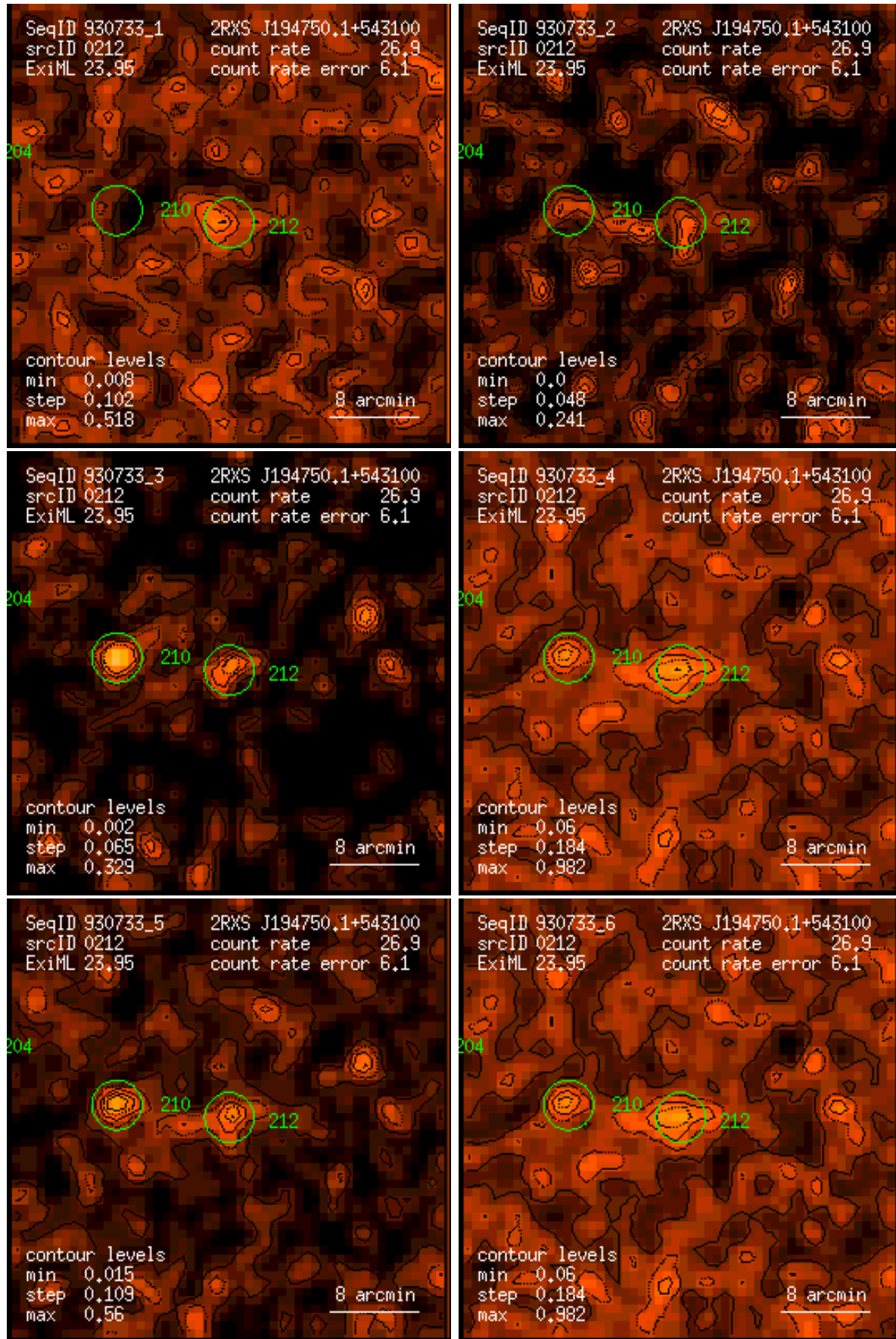
Figure 212: RASS 930733: detection 0212: band rate images, Gaussian filter: (1) PSPC channels 11 – 41, (2) 52 – 90, (3) 91 – 201, (4) 11 – 235, (5) 52 – 201, (6) 11 – 201. Broad band rates in counts/ks. Band rate contour levels in counts/ks/arcmin 2 .
