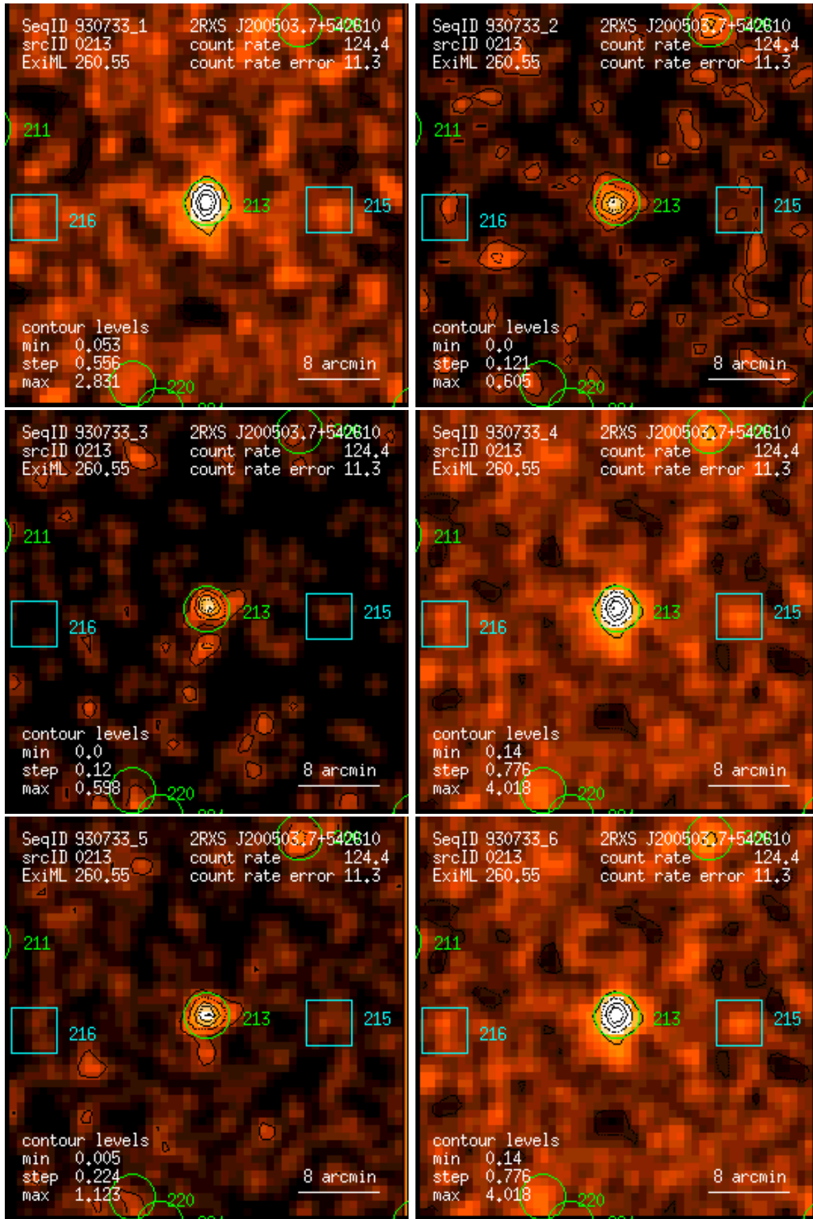
Figure 213: RASS 930733: detection 0213: band rate images, Gaussian filter: (1) PSPC channels 11 – 41, (2) 52 – 90, (3) 91 – 201, (4) 11 – 235, (5) 52 – 201, (6) 11 – 201. Broad band rates in counts/ks. Band rate contour levels in counts/ks/arcmin 2 .
