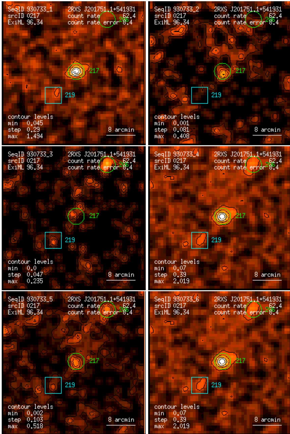
Figure 217: RASS 930733: detection 0217: band rate images, Gaussian filter: (1) PSPC channels 11 – 41, (2) 52 – 90, (3) 91 – 201, (4) 11 – 235, (5) 52 – 201, (6) 11 – 201. Broad band rates in counts/ks. Band rate contour levels in counts/ks/arcmin 2 .
