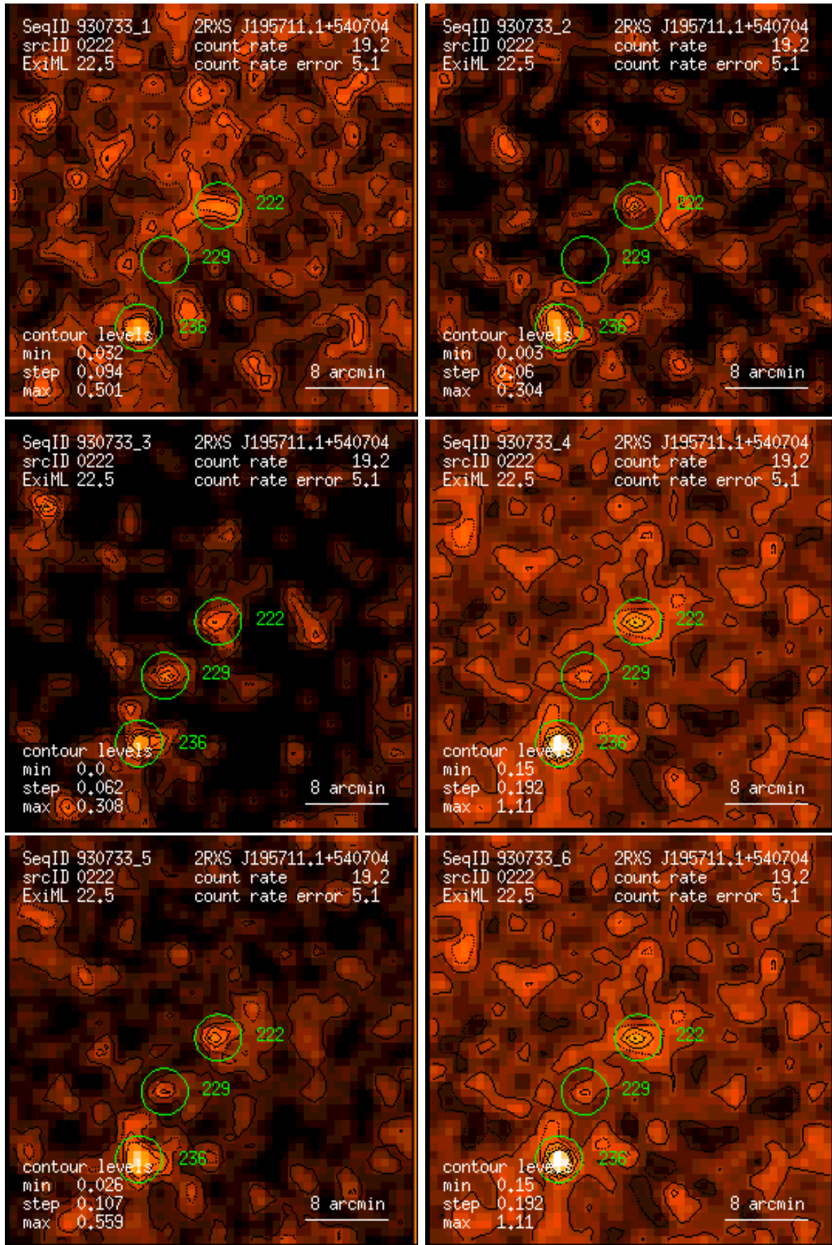
Figure 222: RASS 930733: detection 0222: band rate images, Gaussian filter: (1) PSPC channels 11 – 41, (2) 52 – 90, (3) 91 – 201, (4) 11 – 235, (5) 52 – 201, (6) 11 – 201. Broad band rates in counts/ks. Band rate contour levels in counts/ks/arcmin 2 .
