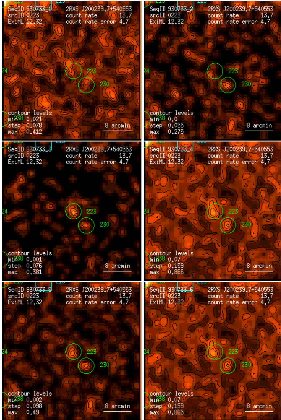
Figure 223: RASS 930733: detection 0223: band rate images, Gaussian filter: (1) PSPC channels 11 – 41, (2) 52 – 90, (3) 91 – 201, (4) 11 – 235, (5) 52 – 201, (6) 11 – 201. Broad band rates in counts/ks. Band rate contour levels in counts/ks/arcmin 2 .
