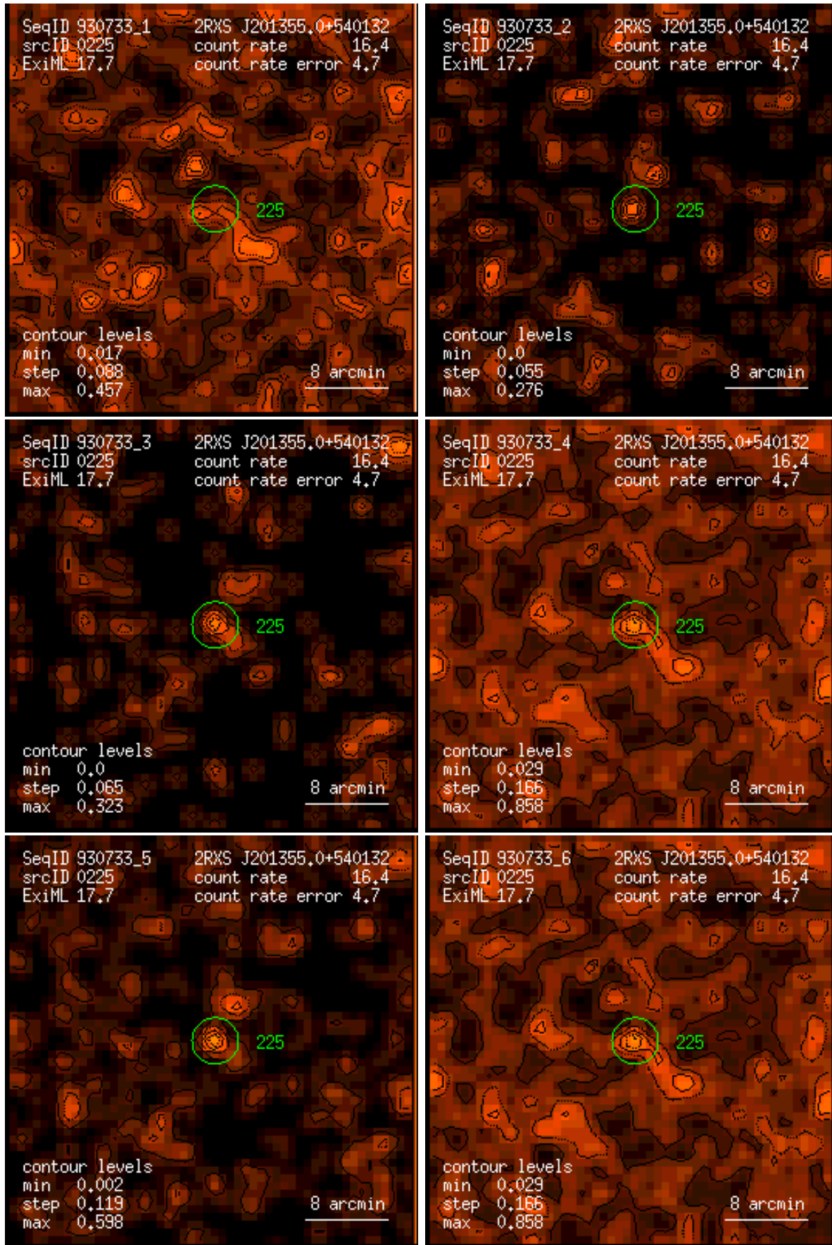
Figure 225: RASS 930733: detection 0225: band rate images, Gaussian filter: (1) PSPC channels 11 – 41, (2) 52 – 90, (3) 91 – 201, (4) 11 – 235, (5) 52 – 201, (6) 11 – 201. Broad band rates in counts/ks. Band rate contour levels in counts/ks/arcmin 2 .
