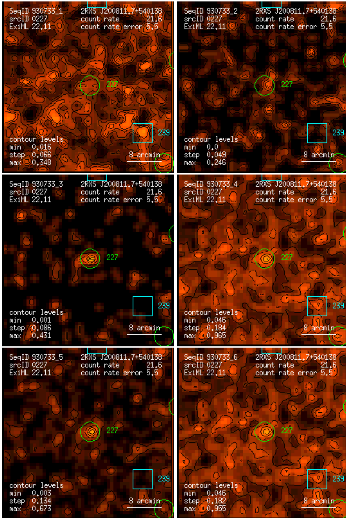
Figure 227: RASS 930733: detection 0227: band rate images, Gaussian filter: (1) PSPC channels 11 – 41, (2) 52 – 90, (3) 91 – 201, (4) 11 – 235, (5) 52 – 201, (6) 11 – 201. Broad band rates in counts/ks. Band rate contour levels in counts/ks/arcmin 2 .
