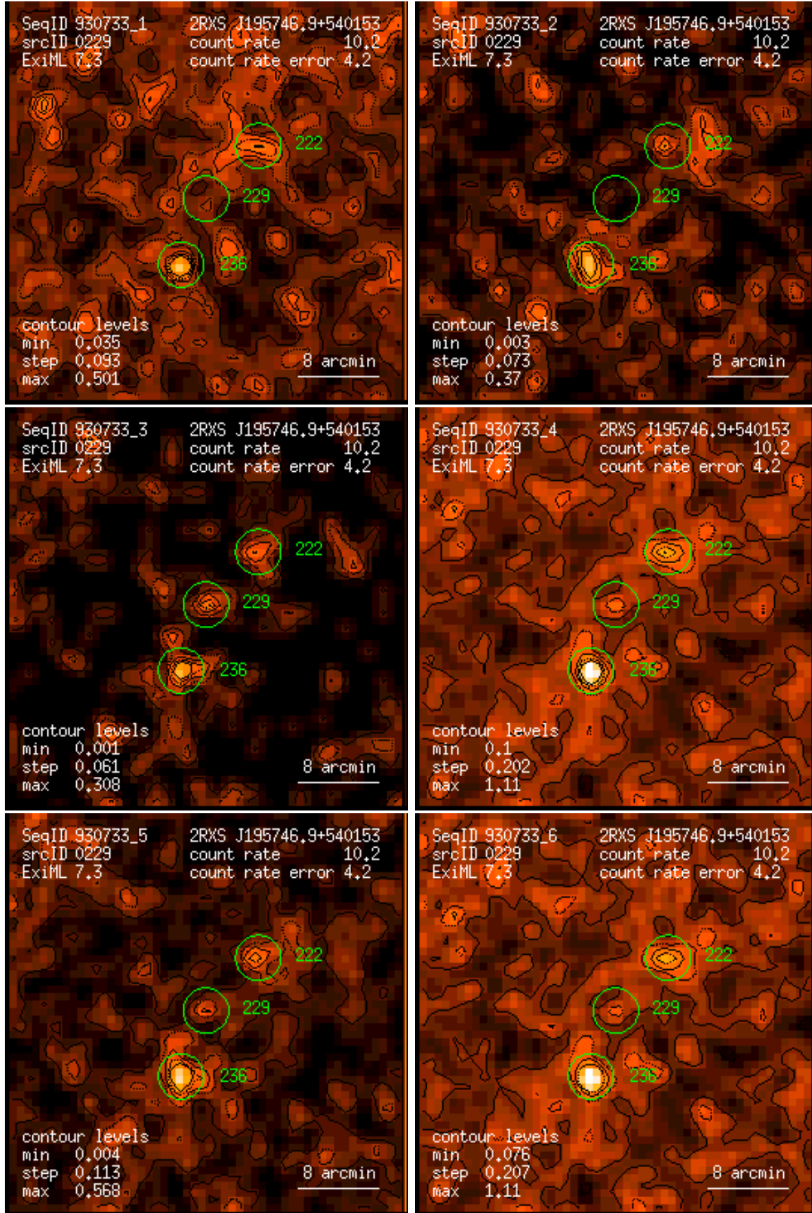
Figure 229: RASS 930733: detection 0229: band rate images, Gaussian filter: (1) PSPC channels 11 – 41, (2) 52 – 90, (3) 91 – 201, (4) 11 – 235, (5) 52 – 201, (6) 11 – 201. Broad band rates in counts/ks. Band rate contour levels in counts/ks/arcmin 2 .
