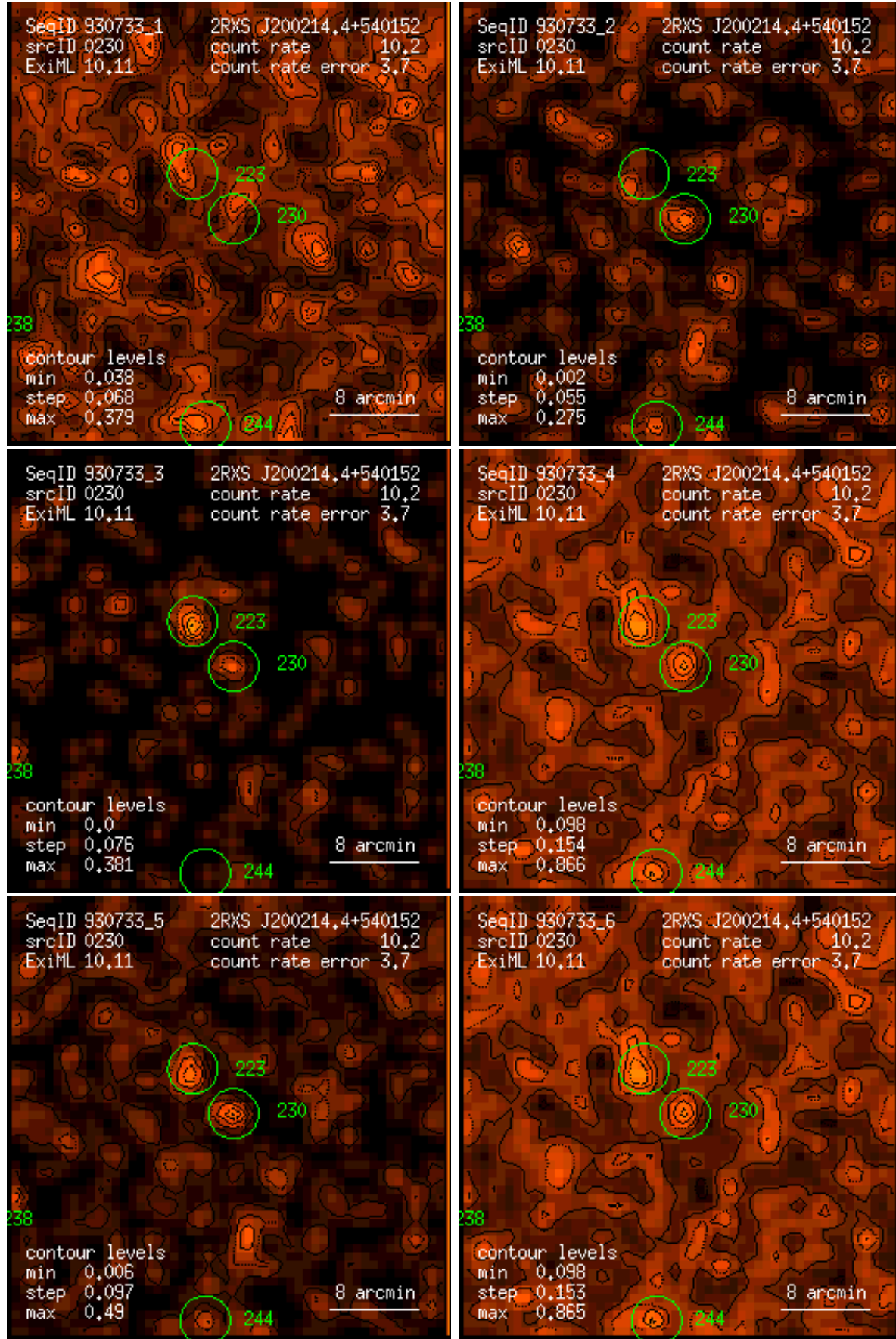
Figure 230: RASS 930733: detection 0230: band rate images, Gaussian filter: (1) PSPC channels 11 – 41, (2) 52 – 90, (3) 91 – 201, (4) 11 – 235, (5) 52 – 201, (6) 11 – 201. Broad band rates in counts/ks. Band rate contour levels in counts/ks/arcmin 2 .
