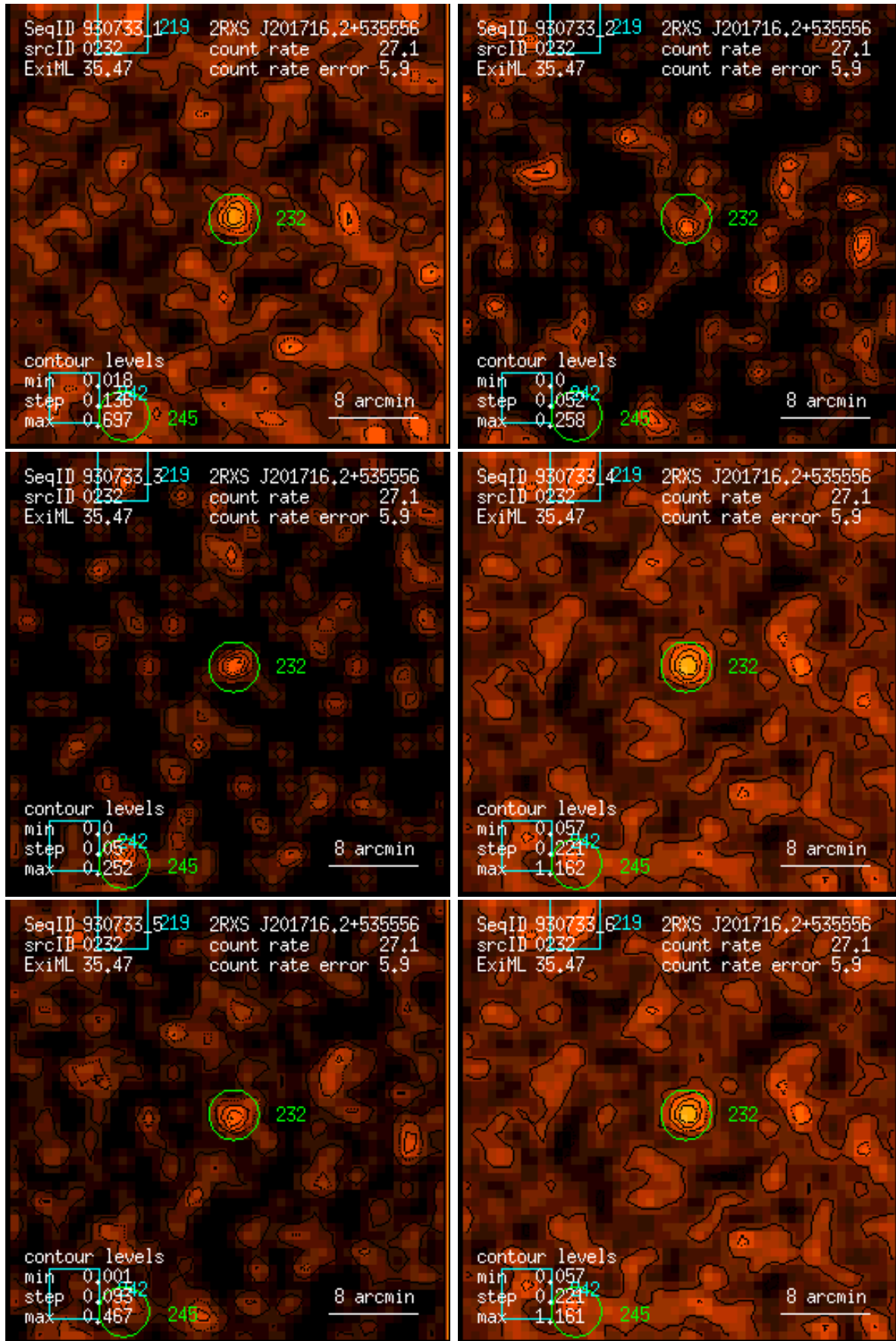
Figure 232: RASS 930733: detection 0232: band rate images, Gaussian filter: (1) PSPC channels 11 – 41, (2) 52 – 90, (3) 91 – 201, (4) 11 – 235, (5) 52 – 201, (6) 11 – 201. Broad band rates in counts/ks. Band rate contour levels in counts/ks/arcmin 2 .
