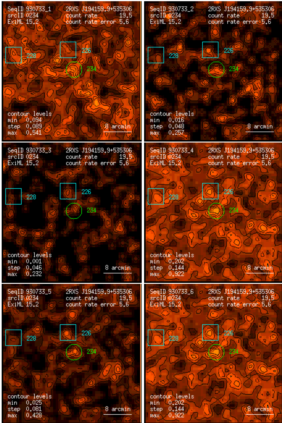
Figure 234: RASS 930733: detection 0234: band rate images, Gaussian filter: (1) PSPC channels 11 – 41, (2) 52 – 90, (3) 91 – 201, (4) 11 – 235, (5) 52 – 201, (6) 11 – 201. Broad band rates in counts/ks. Band rate contour levels in counts/ks/arcmin 2 .
