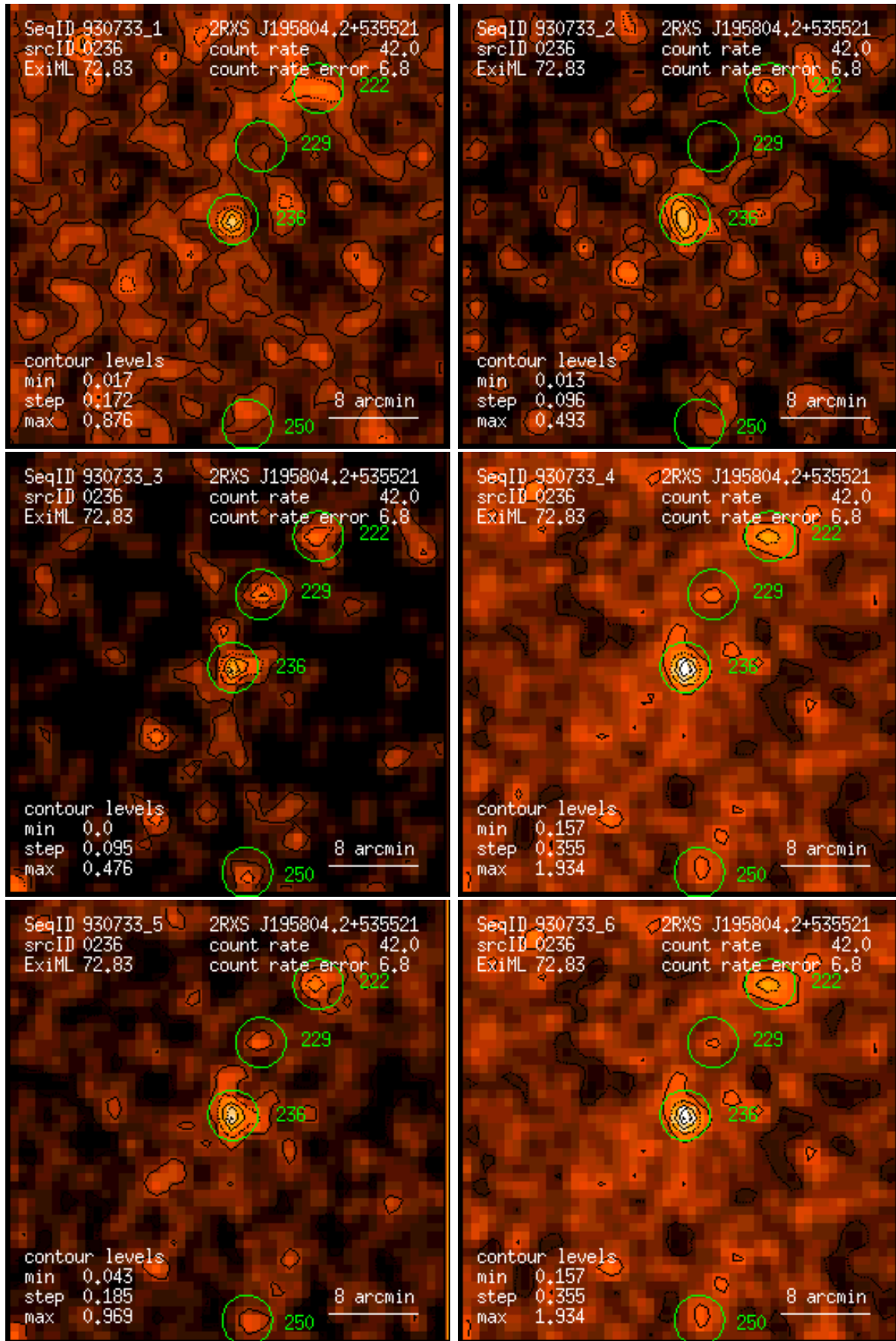
Figure 236: RASS 930733: detection 0236: band rate images, Gaussian filter: (1) PSPC channels 11 – 41, (2) 52 – 90, (3) 91 – 201, (4) 11 – 235, (5) 52 – 201, (6) 11 – 201. Broad band rates in counts/ks. Band rate contour levels in counts/ks/arcmin 2 .
