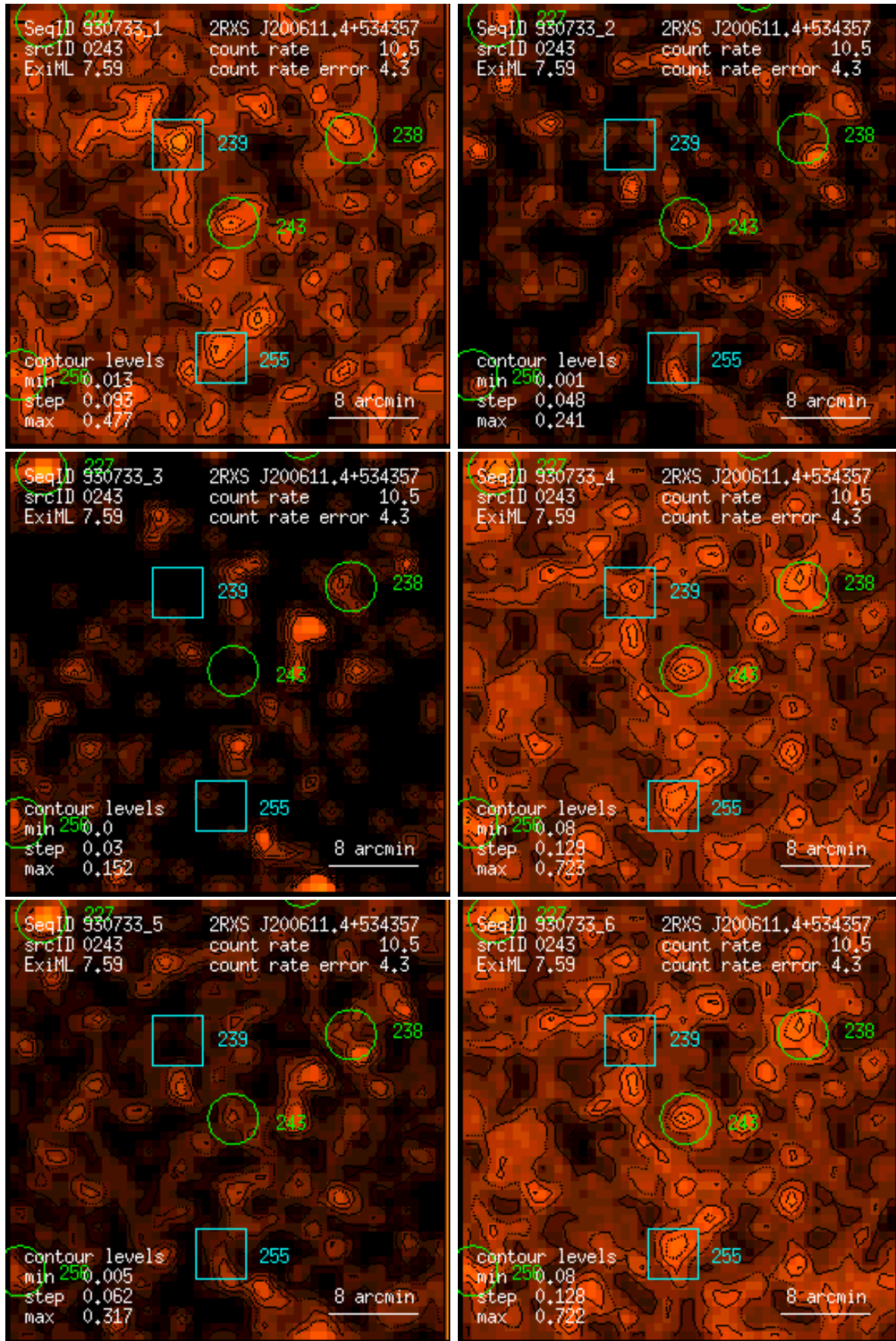
Figure 243: RASS 930733: detection 0243: band rate images, Gaussian filter: (1) PSPC channels 11 – 41, (2) 52 – 90, (3) 91 – 201, (4) 11 – 235, (5) 52 – 201, (6) 11 – 201. Broad band rates in counts/ks. Band rate contour levels in counts/ks/arcmin 2 .
