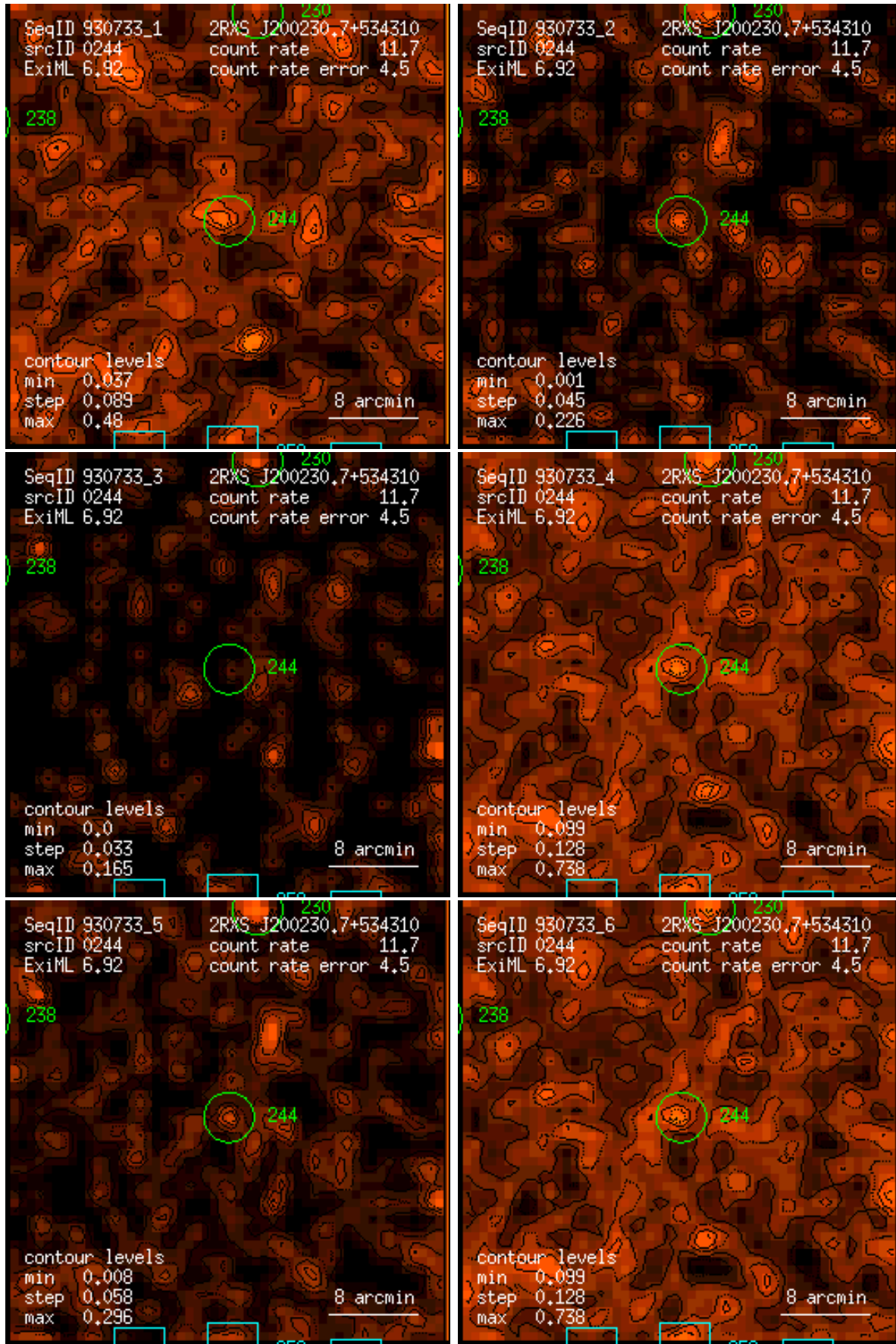
Figure 244: RASS 930733: detection 0244: band rate images, Gaussian filter: (1) PSPC channels 11 – 41, (2) 52 – 90, (3) 91 – 201, (4) 11 – 235, (5) 52 – 201, (6) 11 – 201. Broad band rates in counts/ks. Band rate contour levels in counts/ks/arcmin 2 .
