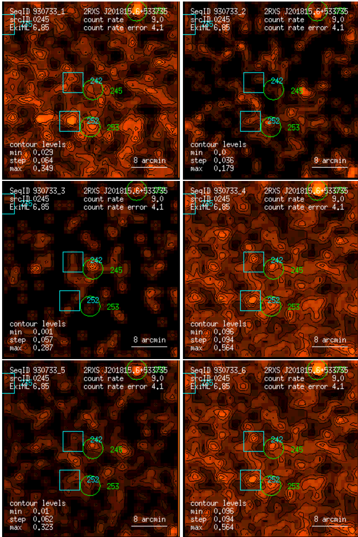
Figure 245: RASS 930733: detection 0245: band rate images, Gaussian filter: (1) PSPC channels 11 – 41, (2) 52 – 90, (3) 91 – 201, (4) 11 – 235, (5) 52 – 201, (6) 11 – 201. Broad band rates in counts/ks. Band rate contour levels in counts/ks/arcmin 2 .
