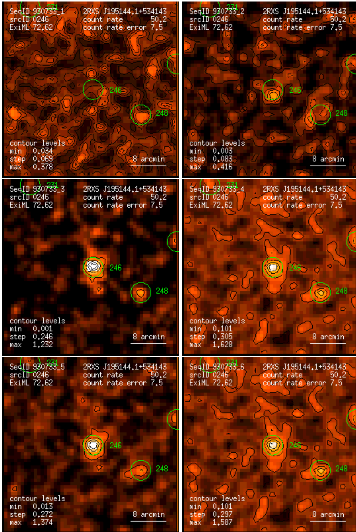
Figure 246: RASS 930733: detection 0246: band rate images, Gaussian filter: (1) PSPC channels 11 – 41, (2) 52 – 90, (3) 91 – 201, (4) 11 – 235, (5) 52 – 201, (6) 11 – 201. Broad band rates in counts/ks. Band rate contour levels in counts/ks/arcmin 2 .
