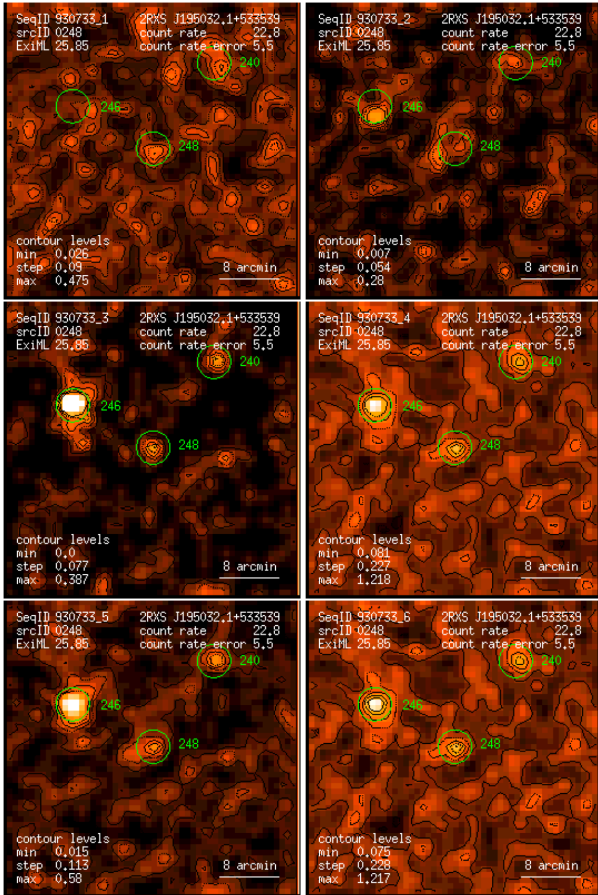
Figure 248: RASS 930733: detection 0248: band rate images, Gaussian filter: (1) PSPC channels 11 – 41, (2) 52 – 90, (3) 91 – 201, (4) 11 – 235, (5) 52 – 201, (6) 11 – 201. Broad band rates in counts/ks. Band rate contour levels in counts/ks/arcmin 2 .
