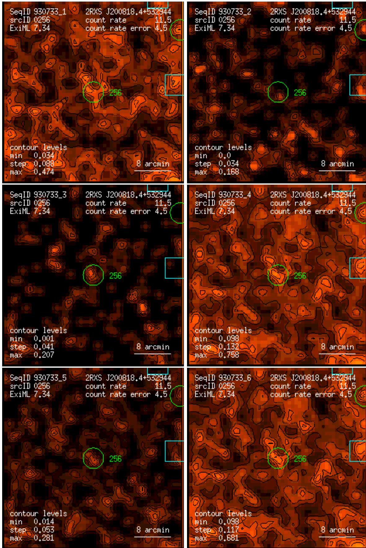
Figure 256: RASS 930733: detection 0256: band rate images, Gaussian filter: (1) PSPC channels 11 – 41, (2) 52 – 90, (3) 91 – 201, (4) 11 – 235, (5) 52 – 201, (6) 11 – 201. Broad band rates in counts/ks. Band rate contour levels in counts/ks/arcmin 2 .
