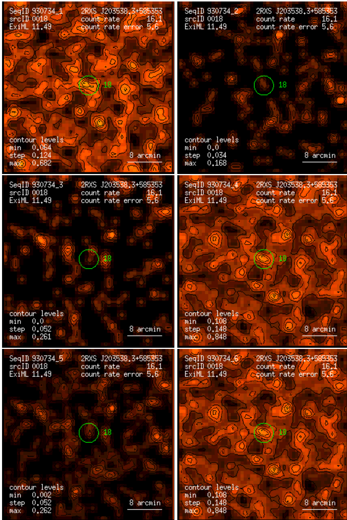
Figure 18: RASS 930734: detection 0018: band rate images, Gaussian filter: (1) PSPC channels 11 – 41, (2) 52 – 90, (3) 91 – 201, (4) 11 – 235, (5) 52 – 201, (6) 11 – 201. Broad band rates in counts/ks. Band rate contour levels in counts/ks/arcmin 2 .
