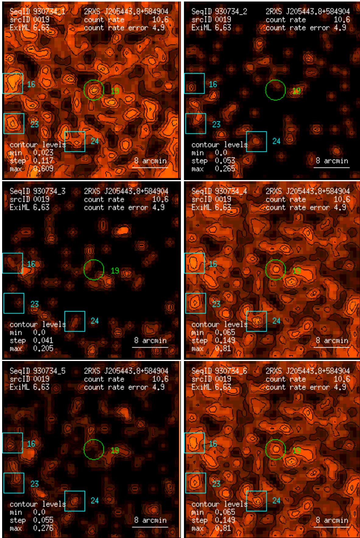
Figure 19: RASS 930734: detection 0019: band rate images, Gaussian filter: (1) PSPC channels 11 – 41, (2) 52 – 90, (3) 91 – 201, (4) 11 – 235, (5) 52 – 201, (6) 11 – 201. Broad band rates in counts/ks. Band rate contour levels in counts/ks/arcmin 2 .
