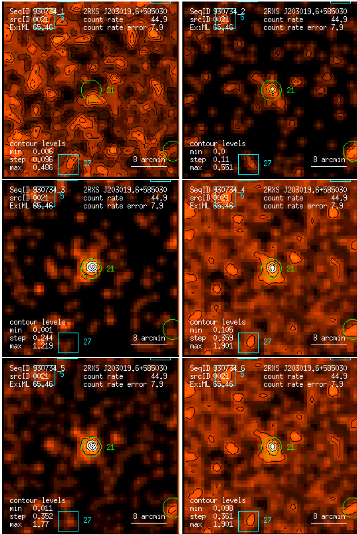
Figure 21: RASS 930734: detection 0021: band rate images, Gaussian filter: (1) PSPC channels 11 – 41, (2) 52 – 90, (3) 91 – 201, (4) 11 – 235, (5) 52 – 201, (6) 11 – 201. Broad band rates in counts/ks. Band rate contour levels in counts/ks/arcmin 2 .
