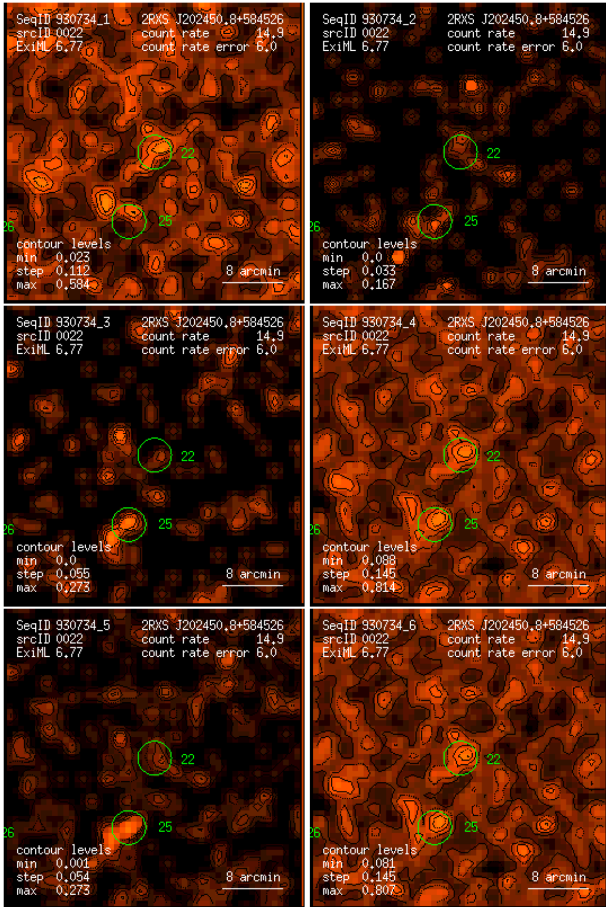
Figure 22: RASS 930734: detection 0022: band rate images, Gaussian filter: (1) PSPC channels 11 – 41, (2) 52 – 90, (3) 91 – 201, (4) 11 – 235, (5) 52 – 201, (6) 11 – 201. Broad band rates in counts/ks. Band rate contour levels in counts/ks/arcmin 2 .
