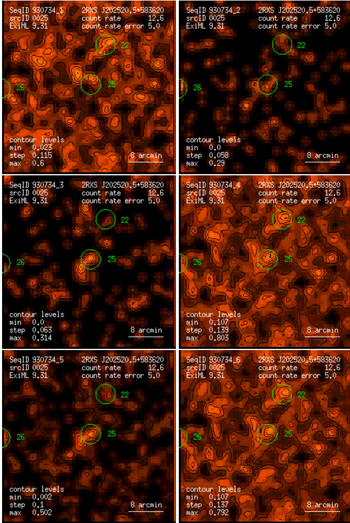
Figure 25: RASS 930734: detection 0025: band rate images, Gaussian filter: (1) PSPC channels 11 – 41, (2) 52 – 90, (3) 91 – 201, (4) 11 – 235, (5) 52 – 201, (6) 11 – 201. Broad band rates in counts/ks. Band rate contour levels in counts/ks/arcmin 2 .
