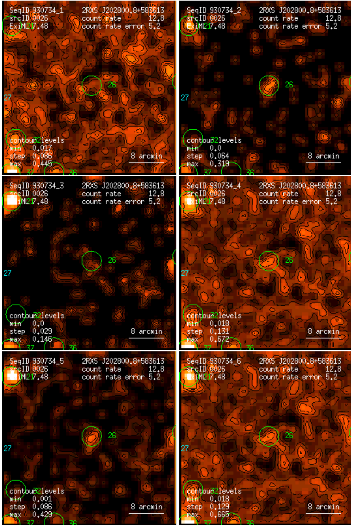
Figure 26: RASS 930734: detection 0026: band rate images, Gaussian filter: (1) PSPC channels 11 – 41, (2) 52 – 90, (3) 91 – 201, (4) 11 – 235, (5) 52 – 201, (6) 11 – 201. Broad band rates in counts/ks. Band rate contour levels in counts/ks/arcmin 2 .
