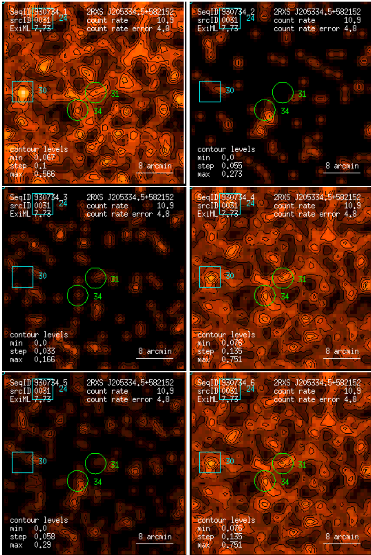
Figure 31: RASS 930734: detection 0031: band rate images, Gaussian filter: (1) PSPC channels 11 – 41, (2) 52 – 90, (3) 91 – 201, (4) 11 – 235, (5) 52 – 201, (6) 11 – 201. Broad band rates in counts/ks. Band rate contour levels in counts/ks/arcmin 2 .
