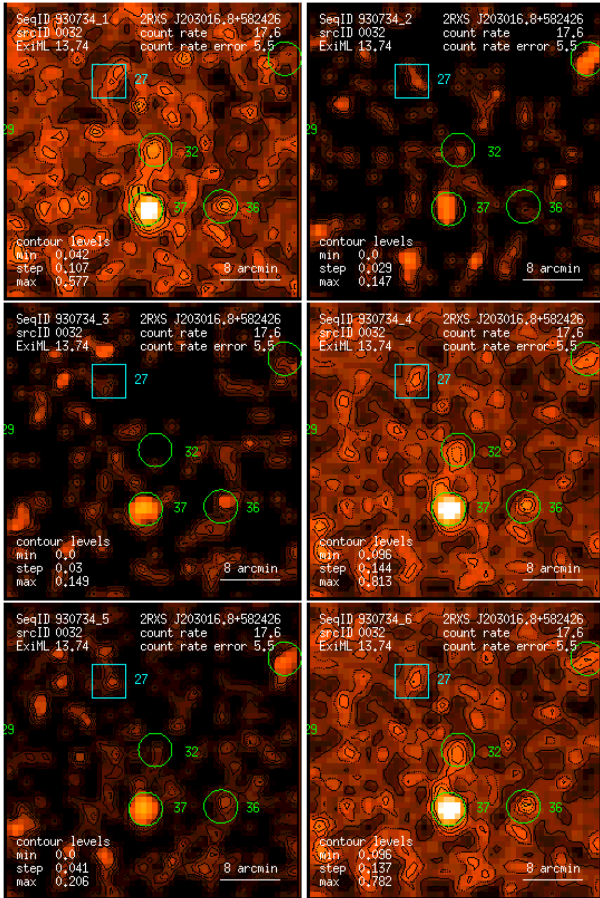
Figure 32: RASS 930734: detection 0032: band rate images, Gaussian filter: (1) PSPC channels 11 – 41, (2) 52 – 90, (3) 91 – 201, (4) 11 – 235, (5) 52 – 201, (6) 11 – 201. Broad band rates in counts/ks. Band rate contour levels in counts/ks/arcmin 2 .
