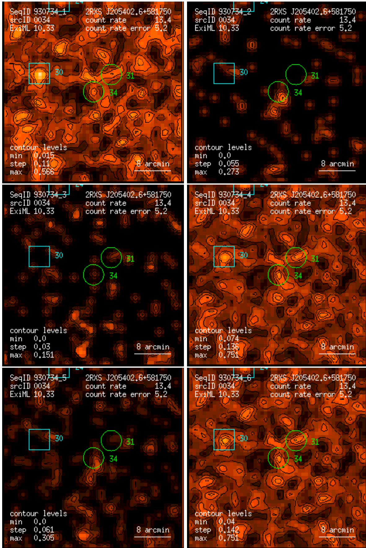
Figure 34: RASS 930734: detection 0034: band rate images, Gaussian filter: (1) PSPC channels 11 – 41, (2) 52 – 90, (3) 91 – 201, (4) 11 – 235, (5) 52 – 201, (6) 11 – 201. Broad band rates in counts/ks. Band rate contour levels in counts/ks/arcmin 2 .
