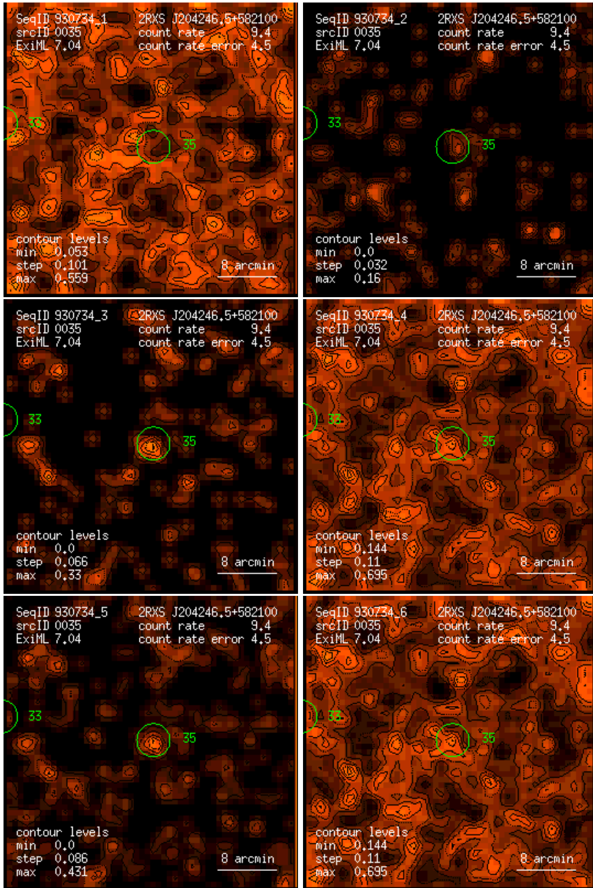
Figure 35: RASS 930734: detection 0035: band rate images, Gaussian filter: (1) PSPC channels 11 – 41, (2) 52 – 90, (3) 91 – 201, (4) 11 – 235, (5) 52 – 201, (6) 11 – 201. Broad band rates in counts/ks. Band rate contour levels in counts/ks/arcmin 2 .
