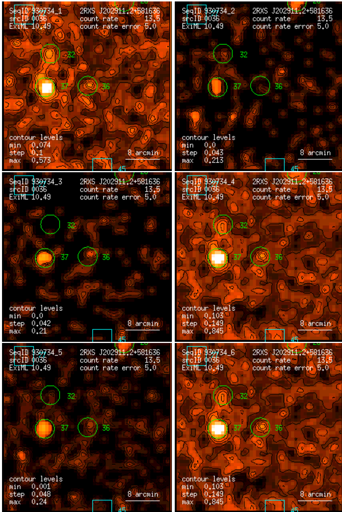
Figure 36: RASS 930734: detection 0036: band rate images, Gaussian filter: (1) PSPC channels 11 – 41, (2) 52 – 90, (3) 91 – 201, (4) 11 – 235, (5) 52 – 201, (6) 11 – 201. Broad band rates in counts/ks. Band rate contour levels in counts/ks/arcmin 2 .
