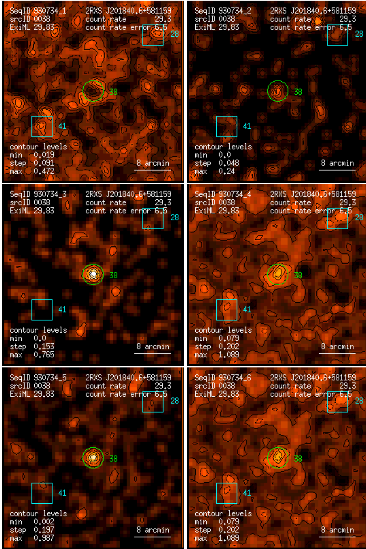
Figure 38: RASS 930734: detection 0038: band rate images, Gaussian filter: (1) PSPC channels 11 – 41, (2) 52 – 90, (3) 91 – 201, (4) 11 – 235, (5) 52 – 201, (6) 11 – 201. Broad band rates in counts/ks. Band rate contour levels in counts/ks/arcmin 2 .
