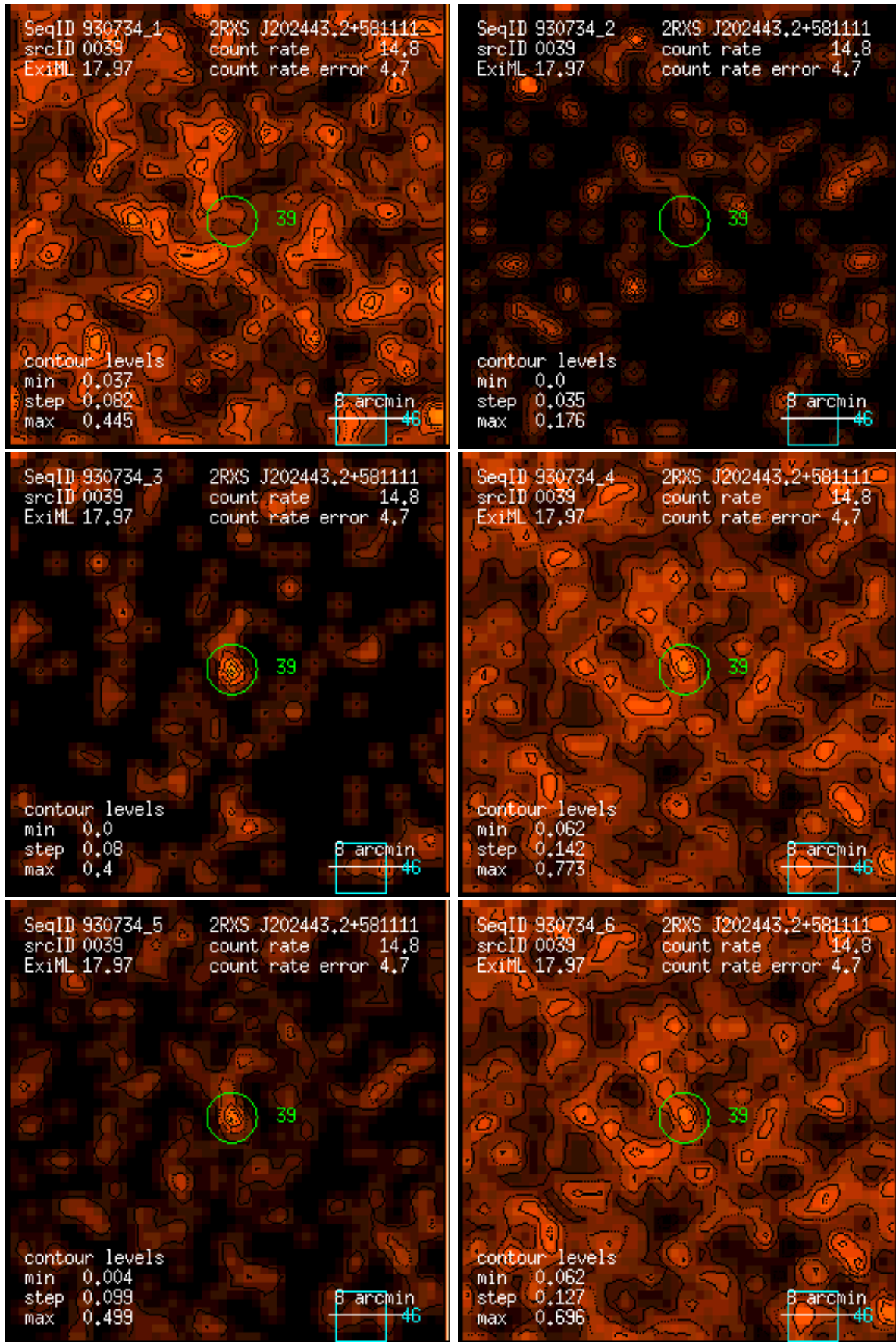
Figure 39: RASS 930734: detection 0039: band rate images, Gaussian filter: (1) PSPC channels 11 – 41, (2) 52 – 90, (3) 91 – 201, (4) 11 – 235, (5) 52 – 201, (6) 11 – 201. Broad band rates in counts/ks. Band rate contour levels in counts/ks/arcmin 2 .
