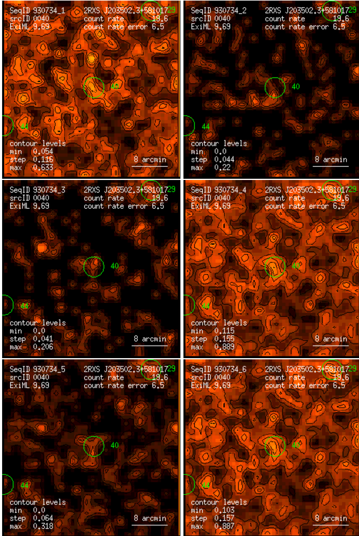
Figure 40: RASS 930734: detection 0040: band rate images, Gaussian filter: (1) PSPC channels 11 – 41, (2) 52 – 90, (3) 91 – 201, (4) 11 – 235, (5) 52 – 201, (6) 11 – 201. Broad band rates in counts/ks. Band rate contour levels in counts/ks/arcmin 2 .
