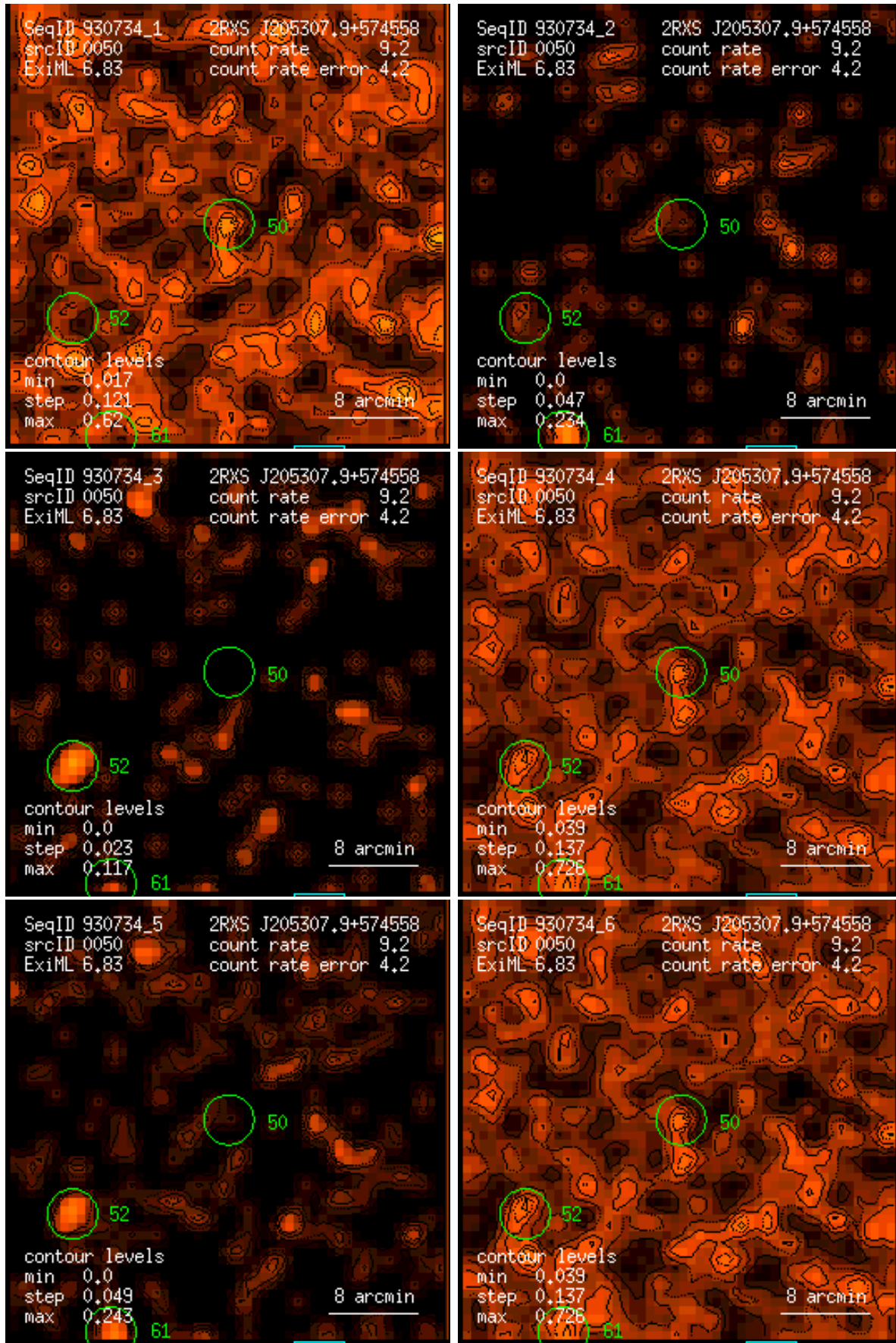
Figure 50: RASS 930734: detection 0050: band rate images, Gaussian filter: (1) PSPC channels 11 – 41, (2) 52 – 90, (3) 91 – 201, (4) 11 – 235, (5) 52 – 201, (6) 11 – 201. Broad band rates in counts/ks. Band rate contour levels in counts/ks/arcmin 2 .
