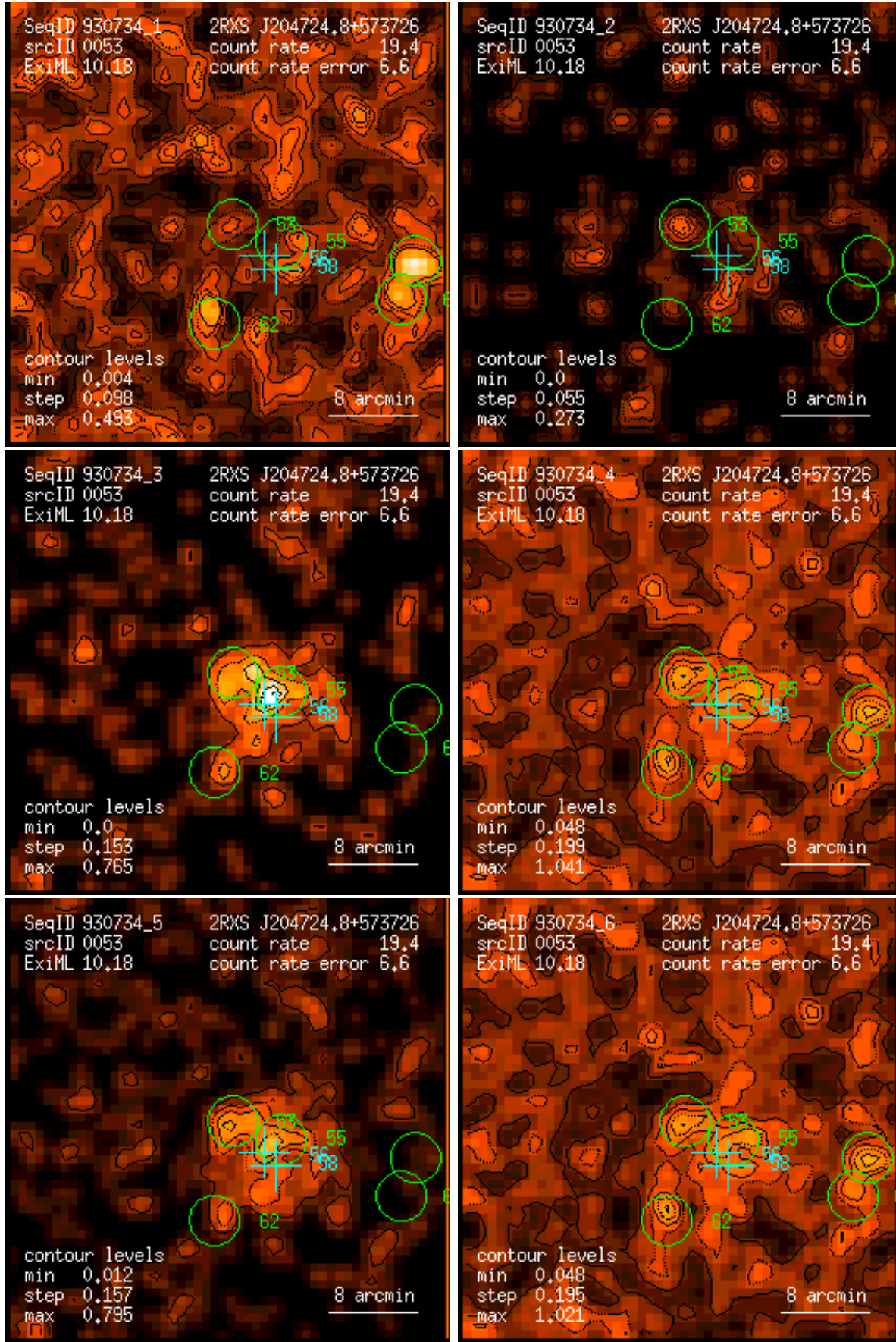
Figure 53: RASS 930734: detection 0053: band rate images, Gaussian filter: (1) PSPC channels 11 – 41, (2) 52 – 90, (3) 91 – 201, (4) 11 – 235, (5) 52 – 201, (6) 11 – 201. Broad band rates in counts/ks. Band rate contour levels in counts/ks/arcmin 2 .
