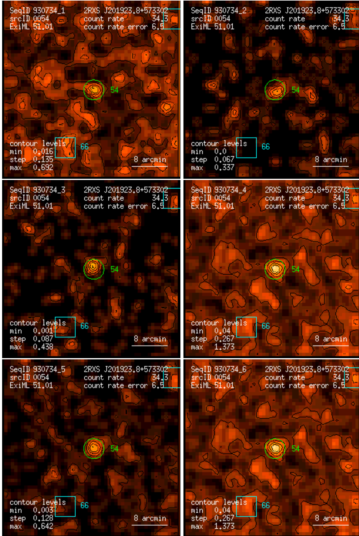
Figure 54: RASS 930734: detection 0054: band rate images, Gaussian filter: (1) PSPC channels 11 – 41, (2) 52 – 90, (3) 91 – 201, (4) 11 – 235, (5) 52 – 201, (6) 11 – 201. Broad band rates in counts/ks. Band rate contour levels in counts/ks/arcmin 2 .
