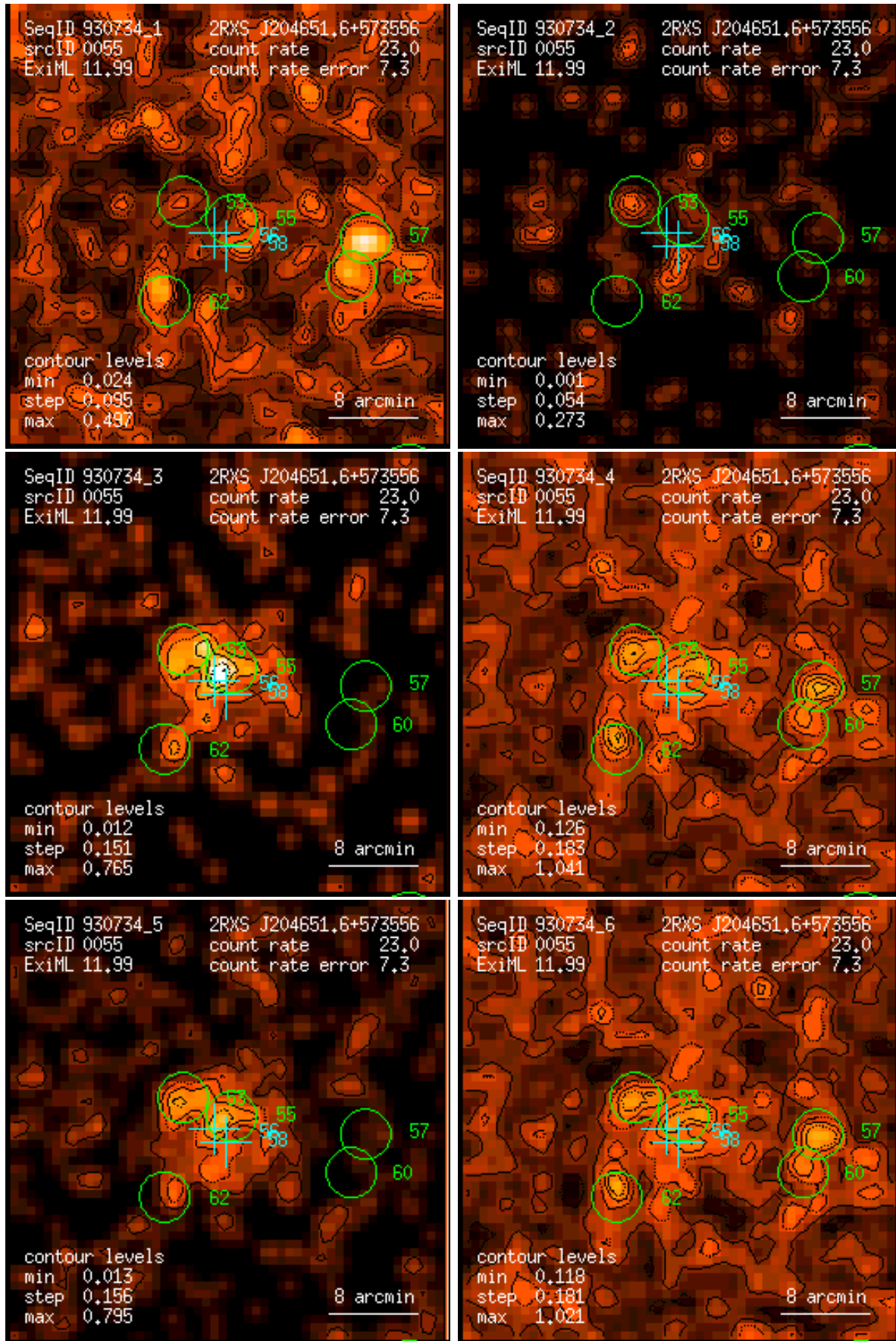
Figure 55: RASS 930734: detection 0055: band rate images, Gaussian filter: (1) PSPC channels 11 – 41, (2) 52 – 90, (3) 91 – 201, (4) 11 – 235, (5) 52 – 201, (6) 11 – 201. Broad band rates in counts/ks. Band rate contour levels in counts/ks/arcmin 2 .
