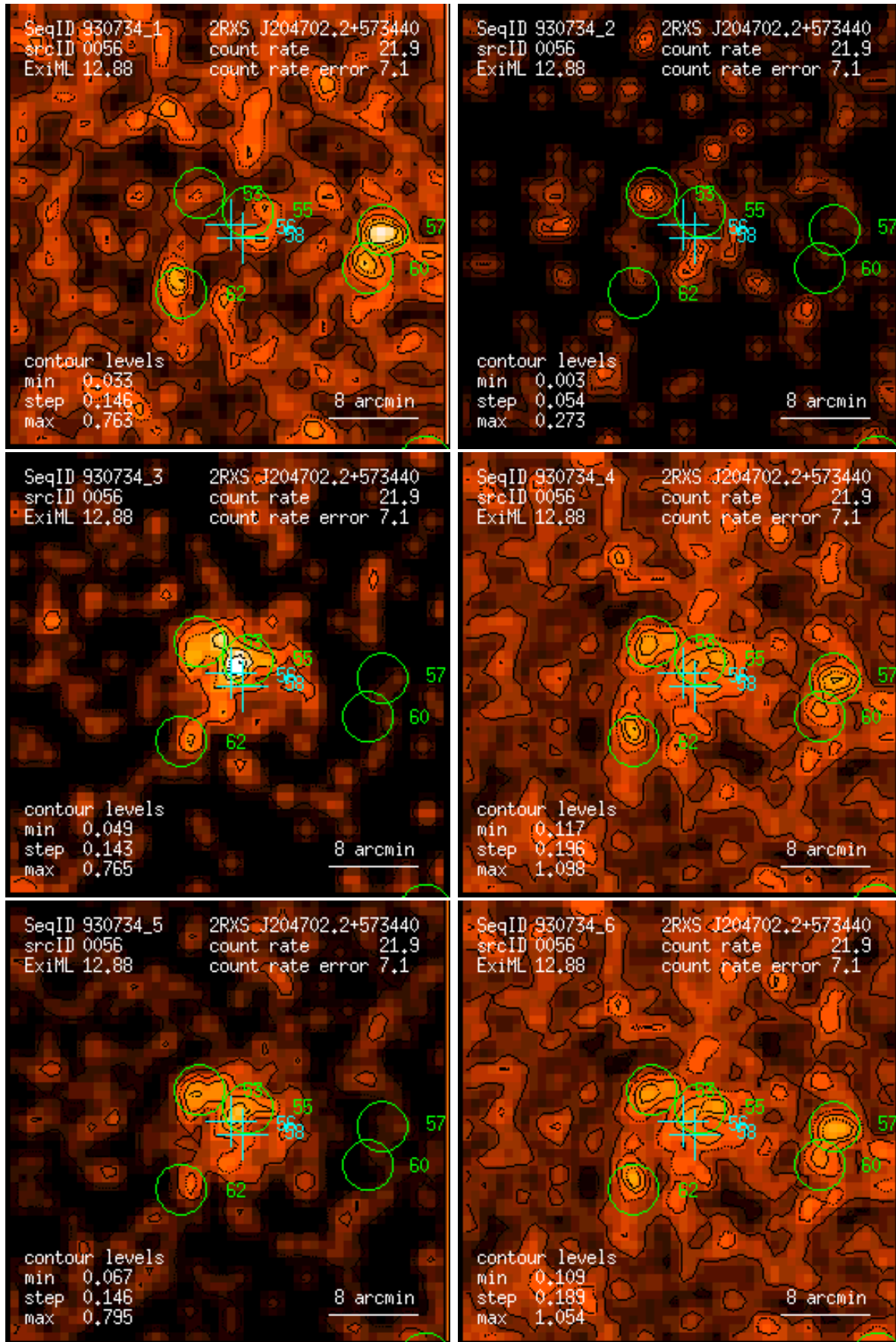
Figure 56: RASS 930734: detection 0056: band rate images, Gaussian filter: (1) PSPC channels 11 – 41, (2) 52 – 90, (3) 91 – 201, (4) 11 – 235, (5) 52 – 201, (6) 11 – 201. Broad band rates in counts/ks. Band rate contour levels in counts/ks/arcmin 2 .
