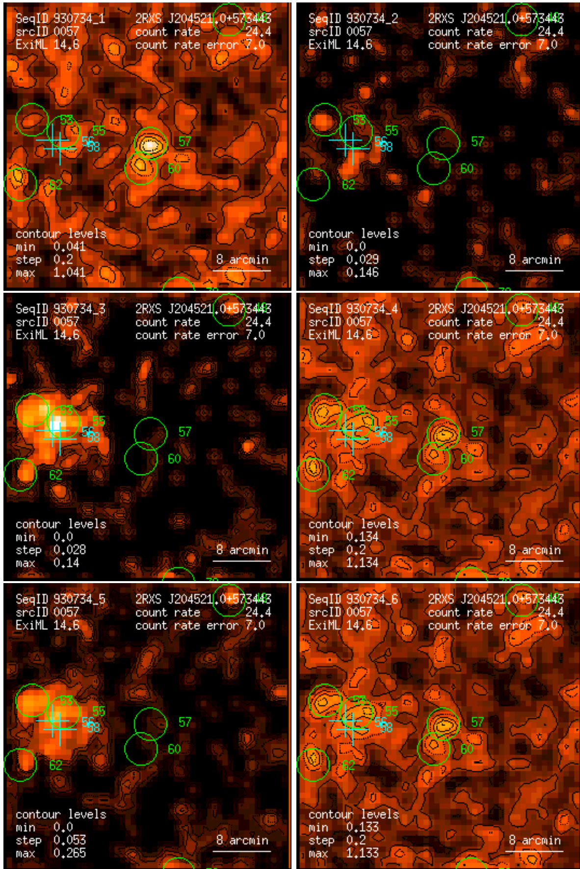
Figure 57: RASS 930734: detection 0057: band rate images, Gaussian filter: (1) PSPC channels 11 – 41, (2) 52 – 90, (3) 91 – 201, (4) 11 – 235, (5) 52 – 201, (6) 11 – 201. Broad band rates in counts/ks. Band rate contour levels in counts/ks/arcmin 2 .
