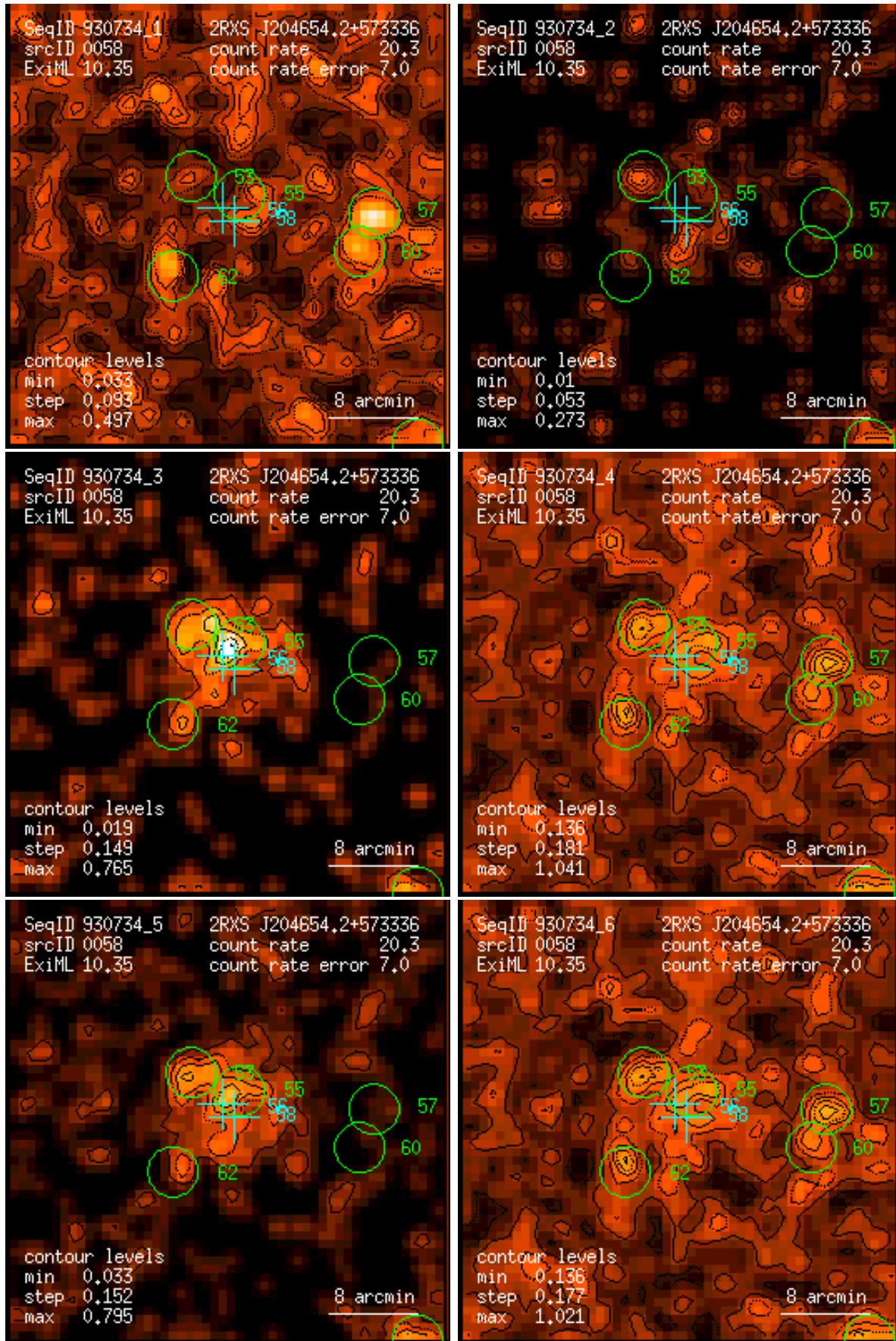
Figure 58: RASS 930734: detection 0058: band rate images, Gaussian filter: (1) PSPC channels 11 – 41, (2) 52 – 90, (3) 91 – 201, (4) 11 – 235, (5) 52 – 201, (6) 11 – 201. Broad band rates in counts/ks. Band rate contour levels in counts/ks/arcmin 2 .
