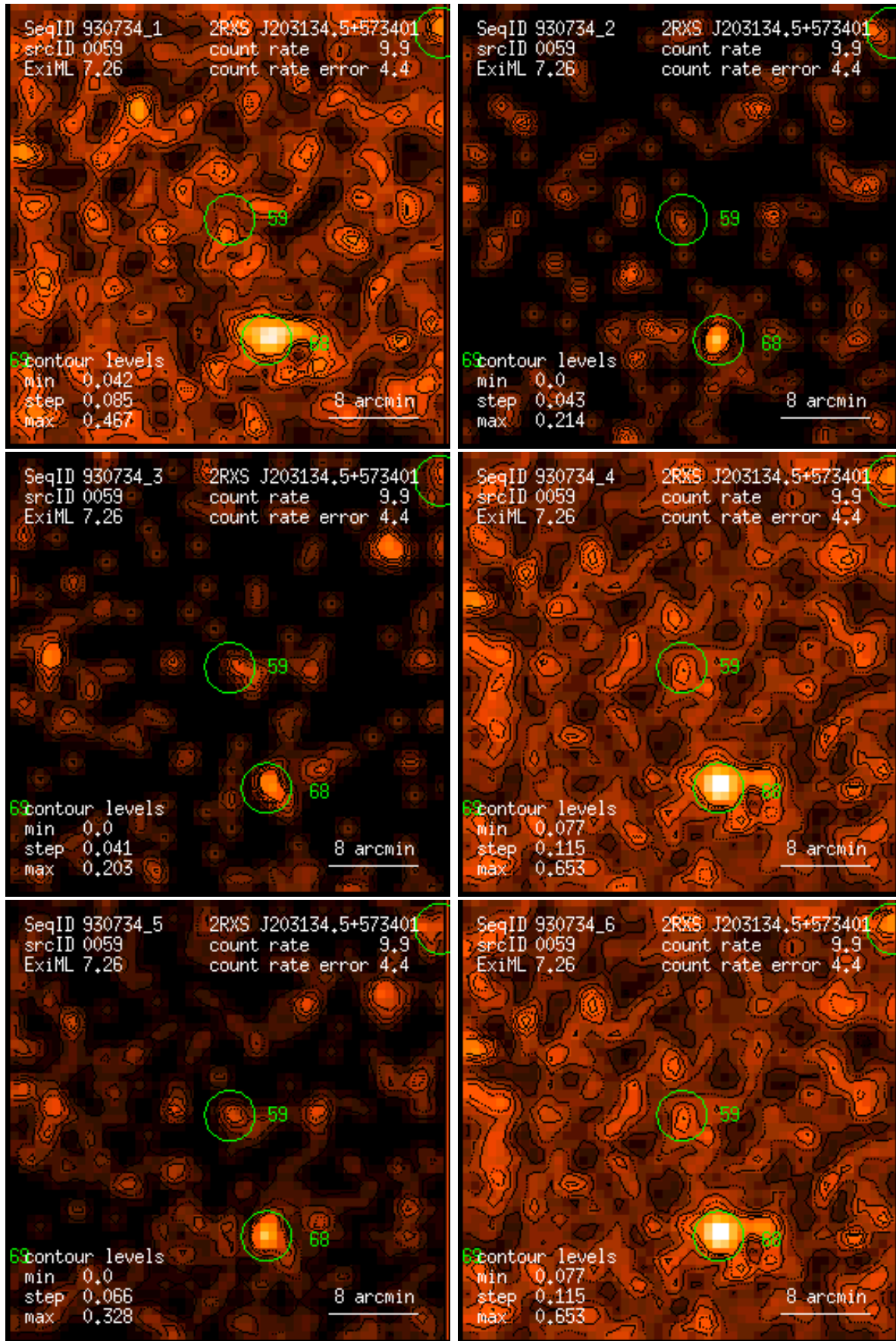
Figure 59: RASS 930734: detection 0059: band rate images, Gaussian filter: (1) PSPC channels 11 – 41, (2) 52 – 90, (3) 91 – 201, (4) 11 – 235, (5) 52 – 201, (6) 11 – 201. Broad band rates in counts/ks. Band rate contour levels in counts/ks/arcmin 2 .
