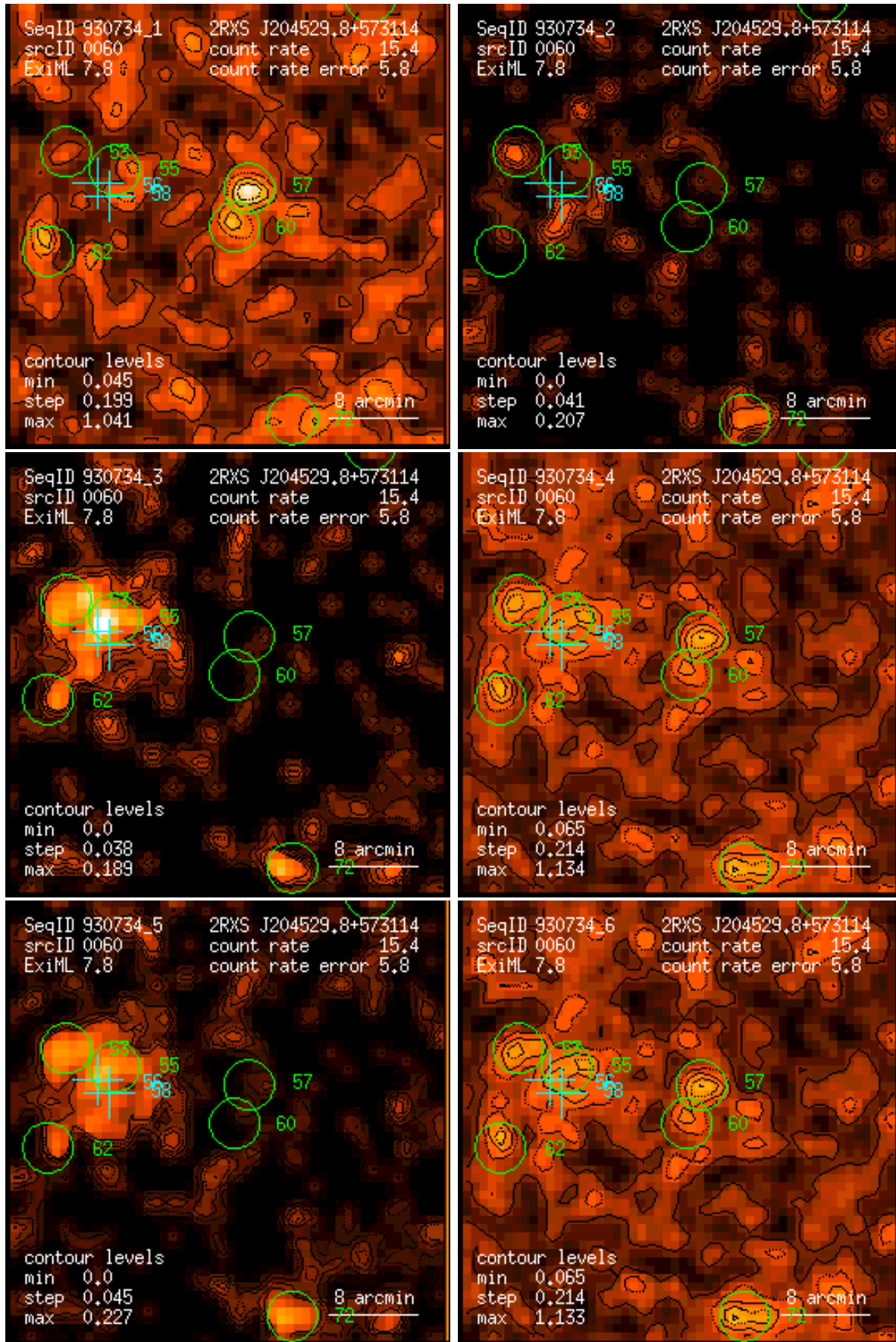
Figure 60: RASS 930734: detection 0060: band rate images, Gaussian filter: (1) PSPC channels 11 – 41, (2) 52 – 90, (3) 91 – 201, (4) 11 – 235, (5) 52 – 201, (6) 11 – 201. Broad band rates in counts/ks. Band rate contour levels in counts/ks/arcmin 2 .
