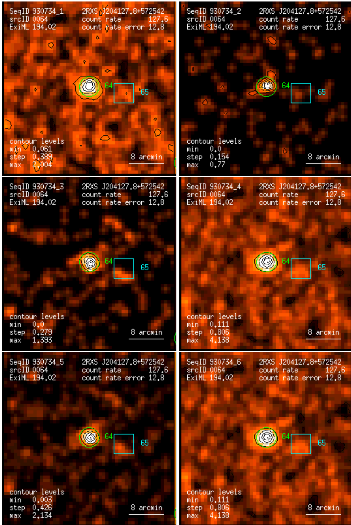
Figure 64: RASS 930734: detection 0064: band rate images, Gaussian filter: (1) PSPC channels 11 – 41, (2) 52 – 90, (3) 91 – 201, (4) 11 – 235, (5) 52 – 201, (6) 11 – 201. Broad band rates in counts/ks. Band rate contour levels in counts/ks/arcmin 2 .
