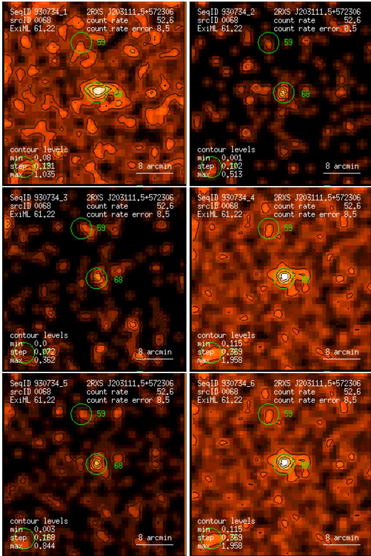
Figure 68: RASS 930734: detection 0068: band rate images, Gaussian filter: (1) PSPC channels 11 – 41, (2) 52 – 90, (3) 91 – 201, (4) 11 – 235, (5) 52 – 201, (6) 11 – 201. Broad band rates in counts/ks. Band rate contour levels in counts/ks/arcmin 2 .
