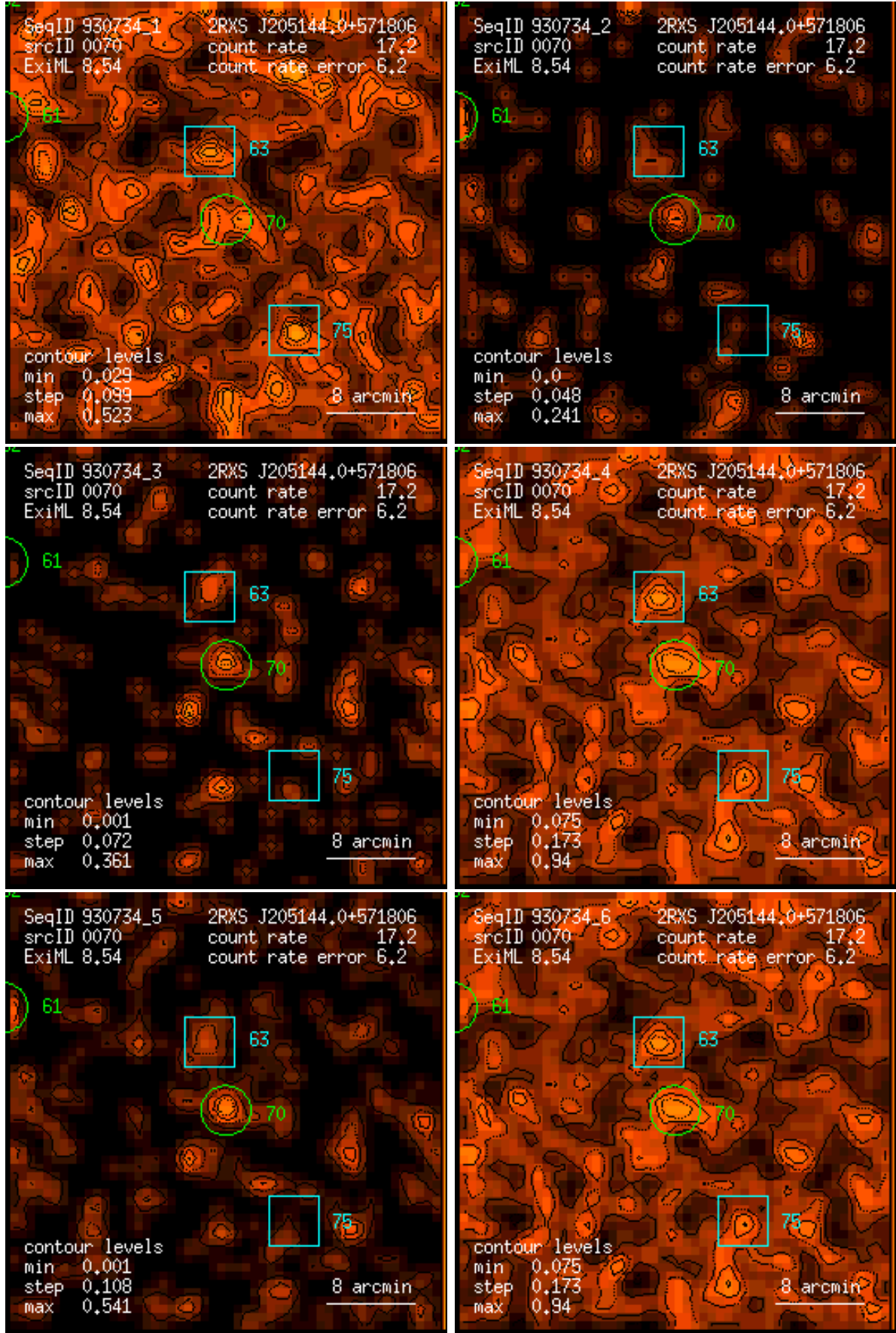
Figure 70: RASS 930734: detection 0070: band rate images, Gaussian filter: (1) PSPC channels 11 – 41, (2) 52 – 90, (3) 91 – 201, (4) 11 – 235, (5) 52 – 201, (6) 11 – 201. Broad band rates in counts/ks. Band rate contour levels in counts/ks/arcmin 2 .
