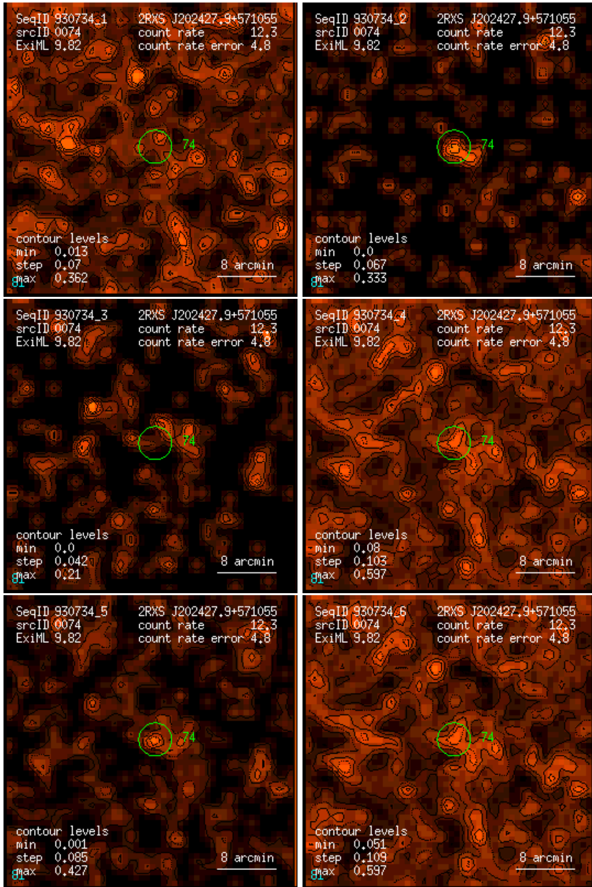
Figure 74: RASS 930734: detection 0074: band rate images, Gaussian filter: (1) PSPC channels 11 – 41, (2) 52 – 90, (3) 91 – 201, (4) 11 – 235, (5) 52 – 201, (6) 11 – 201. Broad band rates in counts/ks. Band rate contour levels in counts/ks/arcmin 2 .
