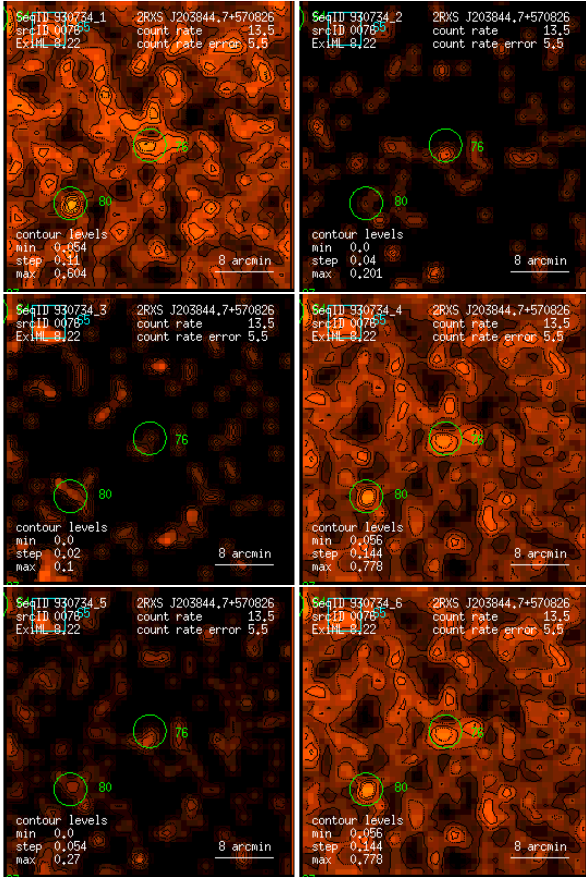
Figure 76: RASS 930734: detection 0076: band rate images, Gaussian filter: (1) PSPC channels 11 – 41, (2) 52 – 90, (3) 91 – 201, (4) 11 – 235, (5) 52 – 201, (6) 11 – 201. Broad band rates in counts/ks. Band rate contour levels in counts/ks/arcmin 2 .
